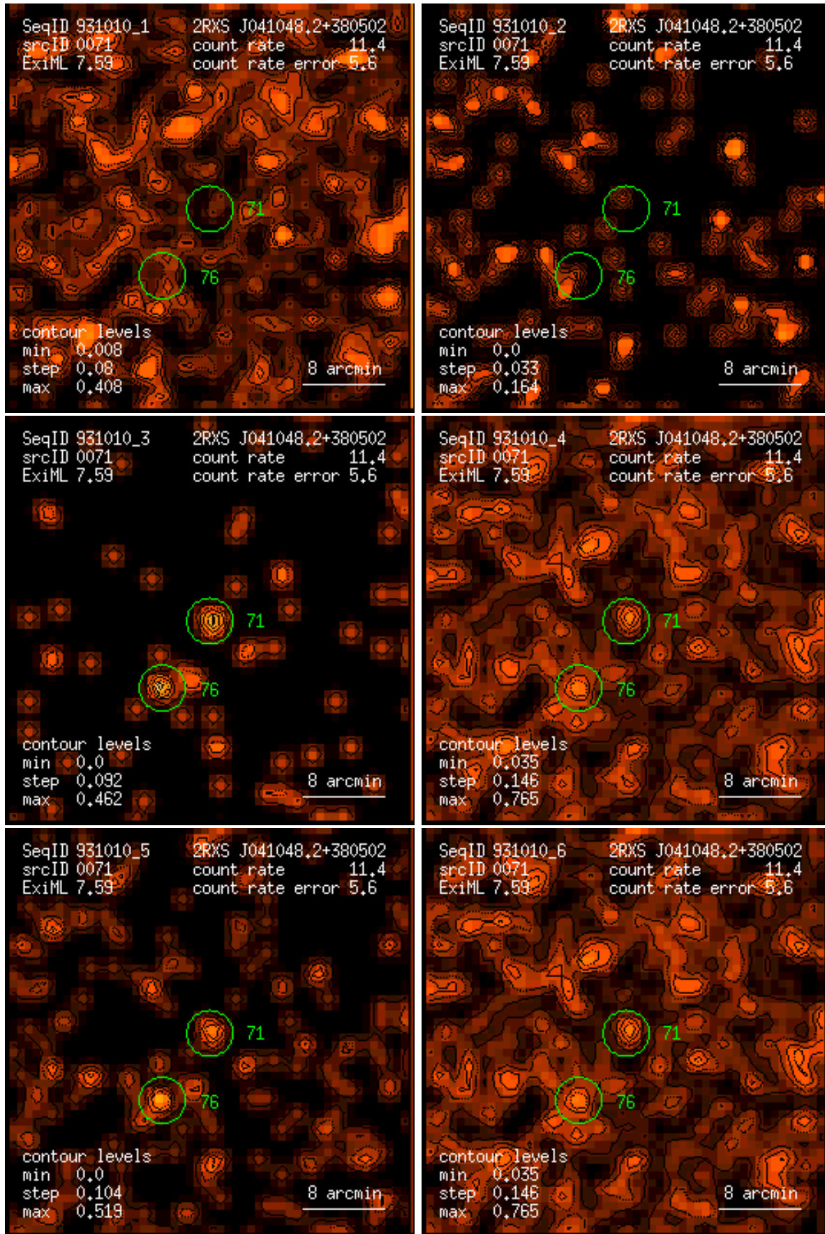
Figure 71: RASS 931010: detection 0071: band rate images, Gaussian filter: (1) PSPC channels 11 – 41, (2) 52 – 90, (3) 91 – 201, (4) 11 – 235, (5) 52 – 201, (6) 11 – 201. Broad band rates in counts/ks. Band rate contour levels in counts/ks/arcmin 2 .
