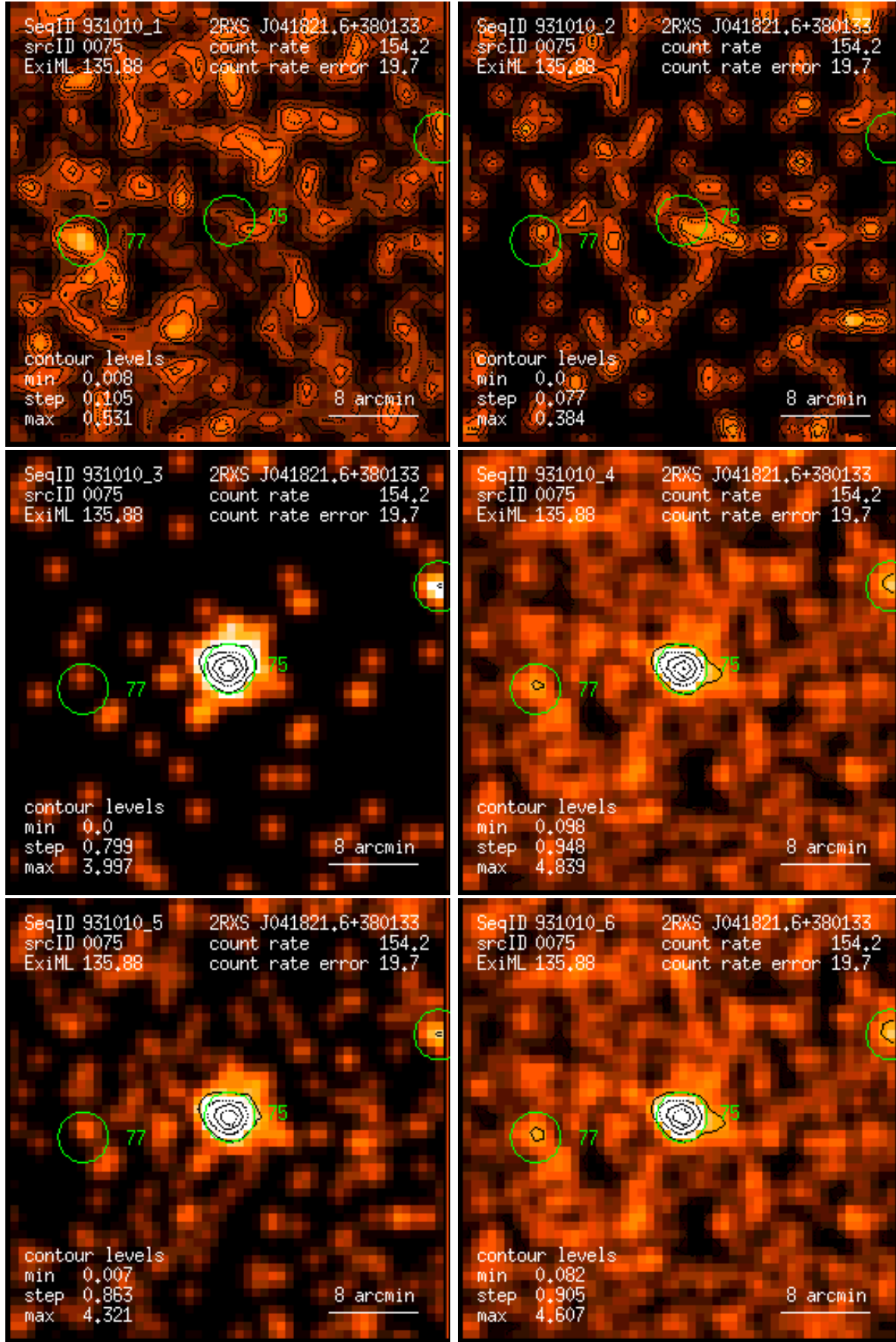
Figure 75: RASS 931010: detection 0075: band rate images, Gaussian filter: (1) PSPC channels 11 – 41, (2) 52 – 90, (3) 91 – 201, (4) 11 – 235, (5) 52 – 201, (6) 11 – 201. Broad band rates in counts/ks. Band rate contour levels in counts/ks/arcmin 2 .
