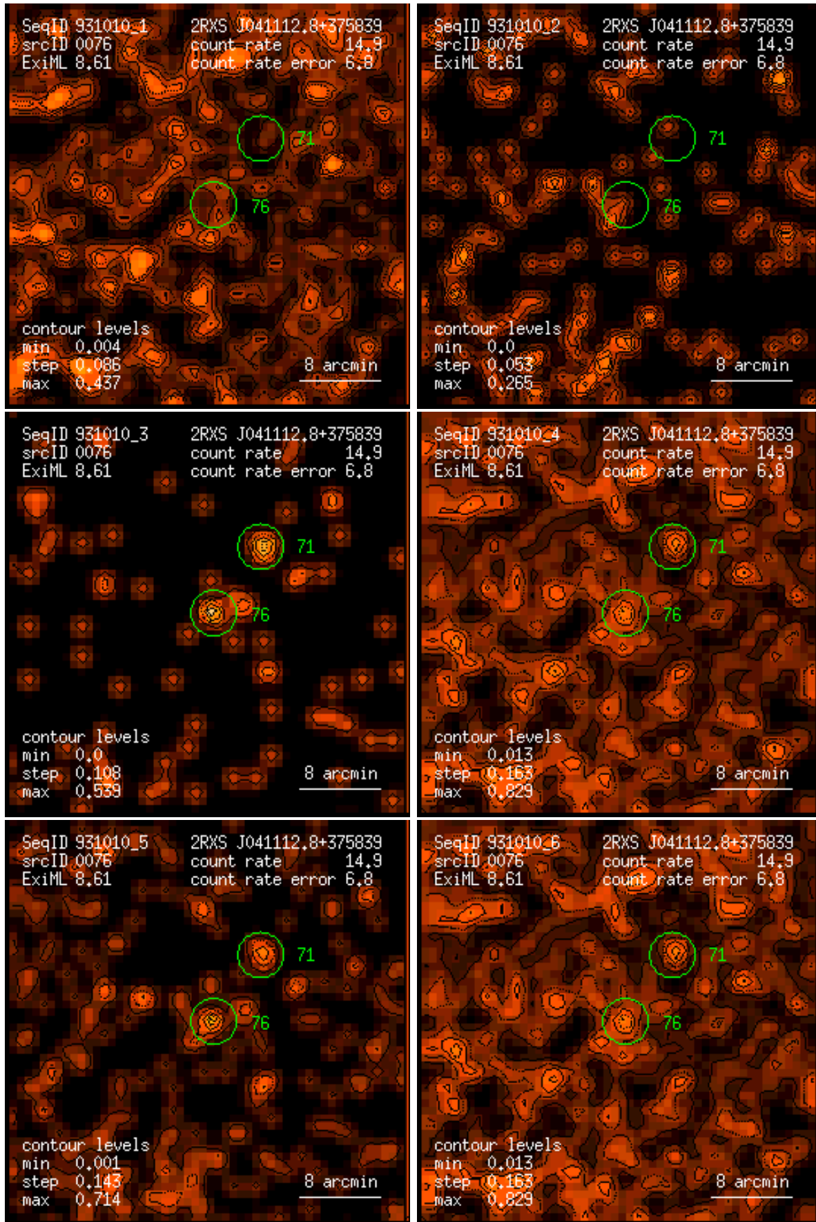
Figure 76: RASS 931010: detection 0076: band rate images, Gaussian filter: (1) PSPC channels 11 – 41, (2) 52 – 90, (3) 91 – 201, (4) 11 – 235, (5) 52 – 201, (6) 11 – 201. Broad band rates in counts/ks. Band rate contour levels in counts/ks/arcmin 2 .
