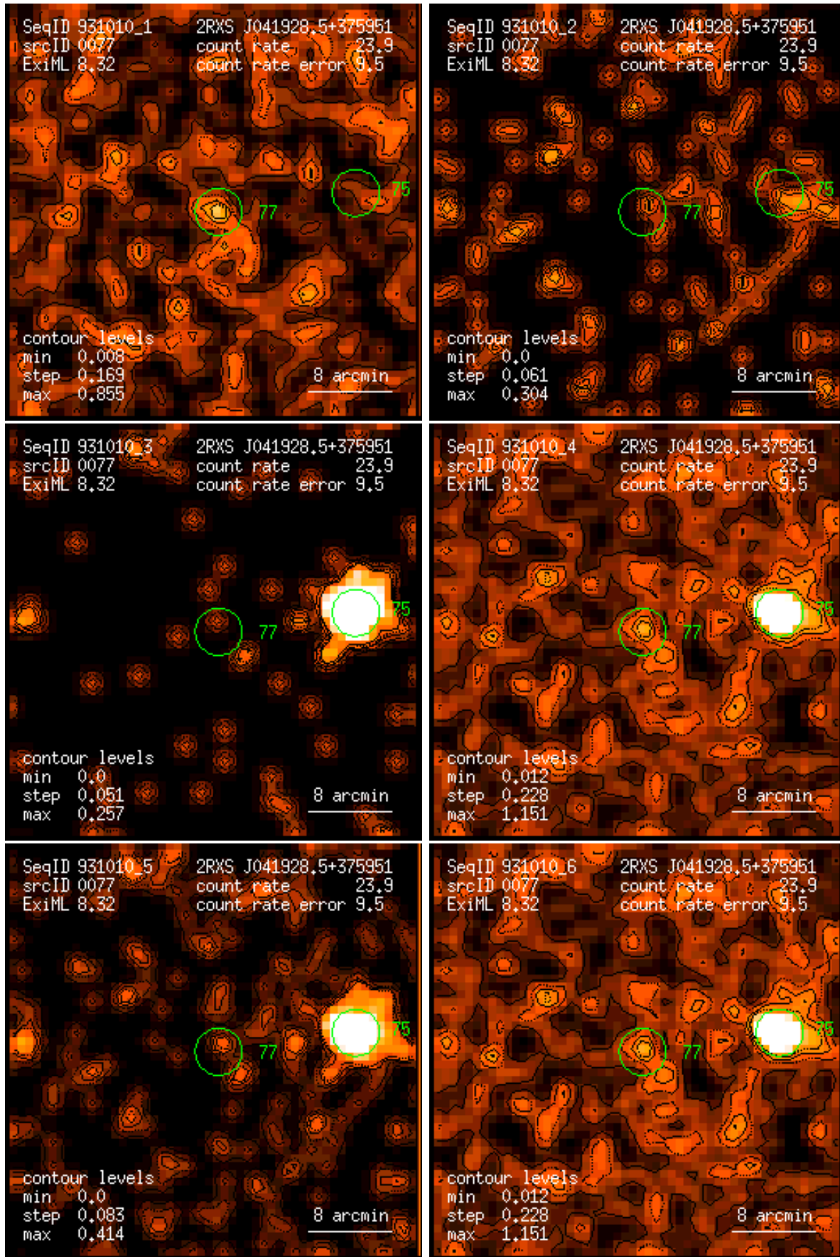
Figure 77: RASS 931010: detection 0077: band rate images, Gaussian filter: (1) PSPC channels 11 – 41, (2) 52 – 90, (3) 91 – 201, (4) 11 – 235, (5) 52 – 201, (6) 11 – 201. Broad band rates in counts/ks. Band rate contour levels in counts/ks/arcmin 2 .
