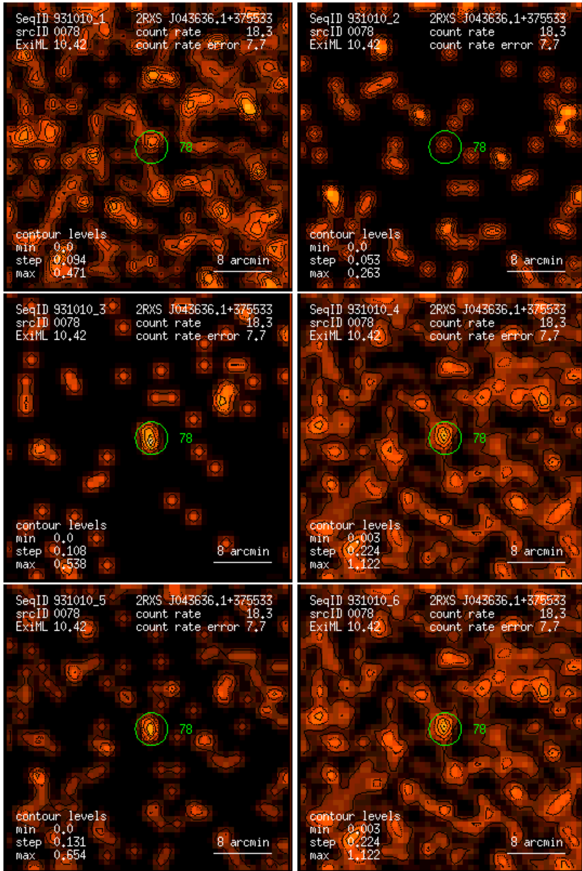
Figure 78: RASS 931010: detection 0078: band rate images, Gaussian filter: (1) PSPC channels 11 – 41, (2) 52 – 90, (3) 91 – 201, (4) 11 – 235, (5) 52 – 201, (6) 11 – 201. Broad band rates in counts/ks. Band rate contour levels in counts/ks/arcmin 2 .
