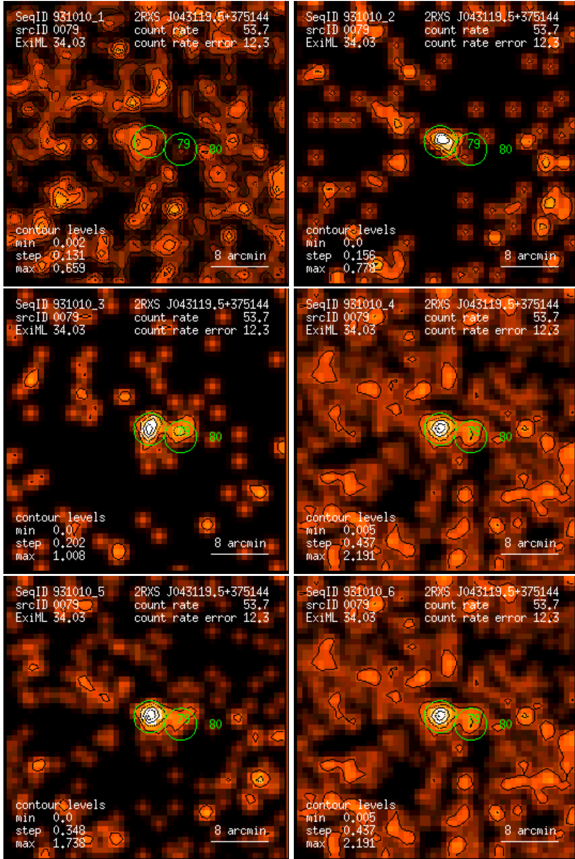
Figure 79: RASS 931010: detection 0079: band rate images, Gaussian filter: (1) PSPC channels 11 – 41, (2) 52 – 90, (3) 91 – 201, (4) 11 – 235, (5) 52 – 201, (6) 11 – 201. Broad band rates in counts/ks. Band rate contour levels in counts/ks/arcmin 2 .
