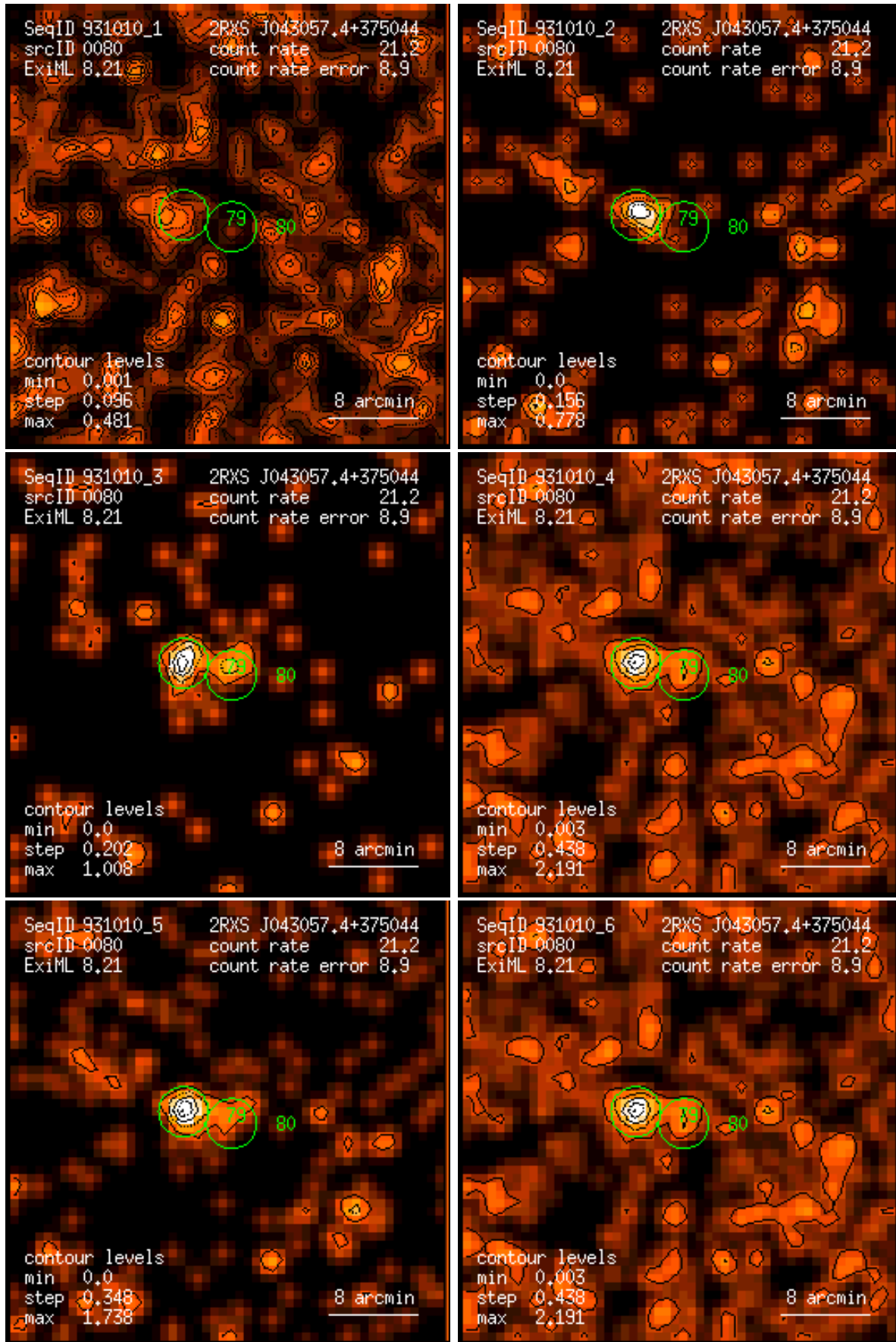
Figure 80: RASS 931010: detection 0080: band rate images, Gaussian filter: (1) PSPC channels 11 – 41, (2) 52 – 90, (3) 91 – 201, (4) 11 – 235, (5) 52 – 201, (6) 11 – 201. Broad band rates in counts/ks. Band rate contour levels in counts/ks/arcmin 2 .
