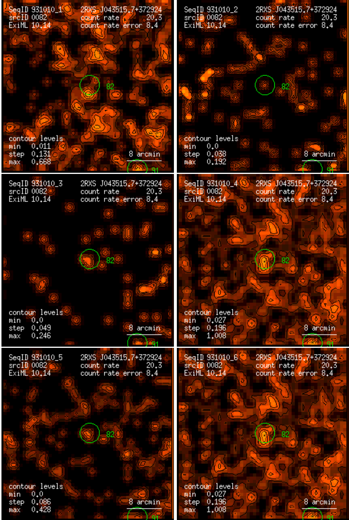
Figure 82: RASS 931010: detection 0082: band rate images, Gaussian filter: (1) PSPC channels 11 – 41, (2) 52 – 90, (3) 91 – 201, (4) 11 – 235, (5) 52 – 201, (6) 11 – 201. Broad band rates in counts/ks. Band rate contour levels in counts/ks/arcmin 2 .
