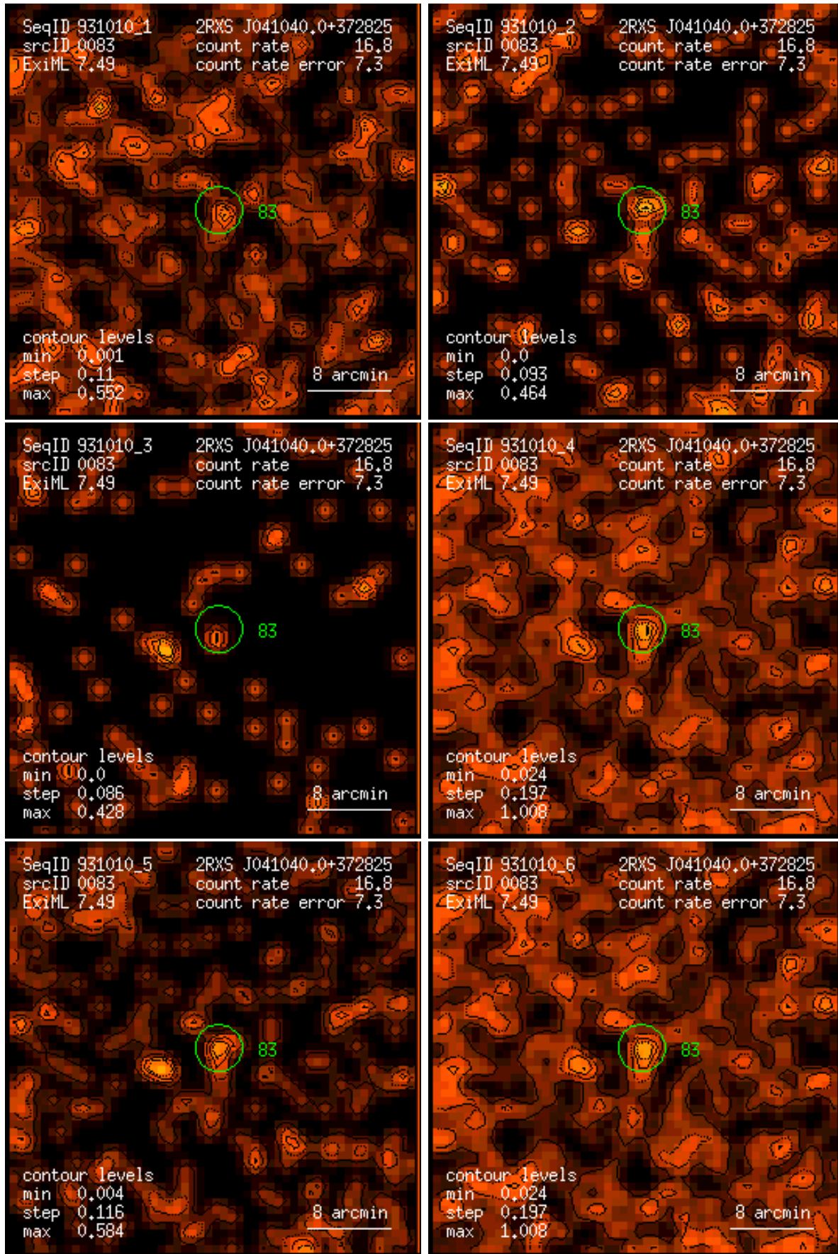
Figure 83: RASS 931010: detection 0083: band rate images, Gaussian filter: (1) PSPC channels 11 – 41, (2) 52 – 90, (3) 91 – 201, (4) 11 – 235, (5) 52 – 201, (6) 11 – 201. Broad band rates in counts/ks. Band rate contour levels in counts/ks/arcmin 2 .
