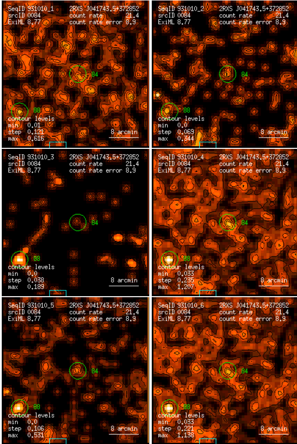
Figure 84: RASS 931010: detection 0084: band rate images, Gaussian filter: (1) PSPC channels 11 – 41, (2) 52 – 90, (3) 91 – 201, (4) 11 – 235, (5) 52 – 201, (6) 11 – 201. Broad band rates in counts/ks. Band rate contour levels in counts/ks/arcmin 2 .
