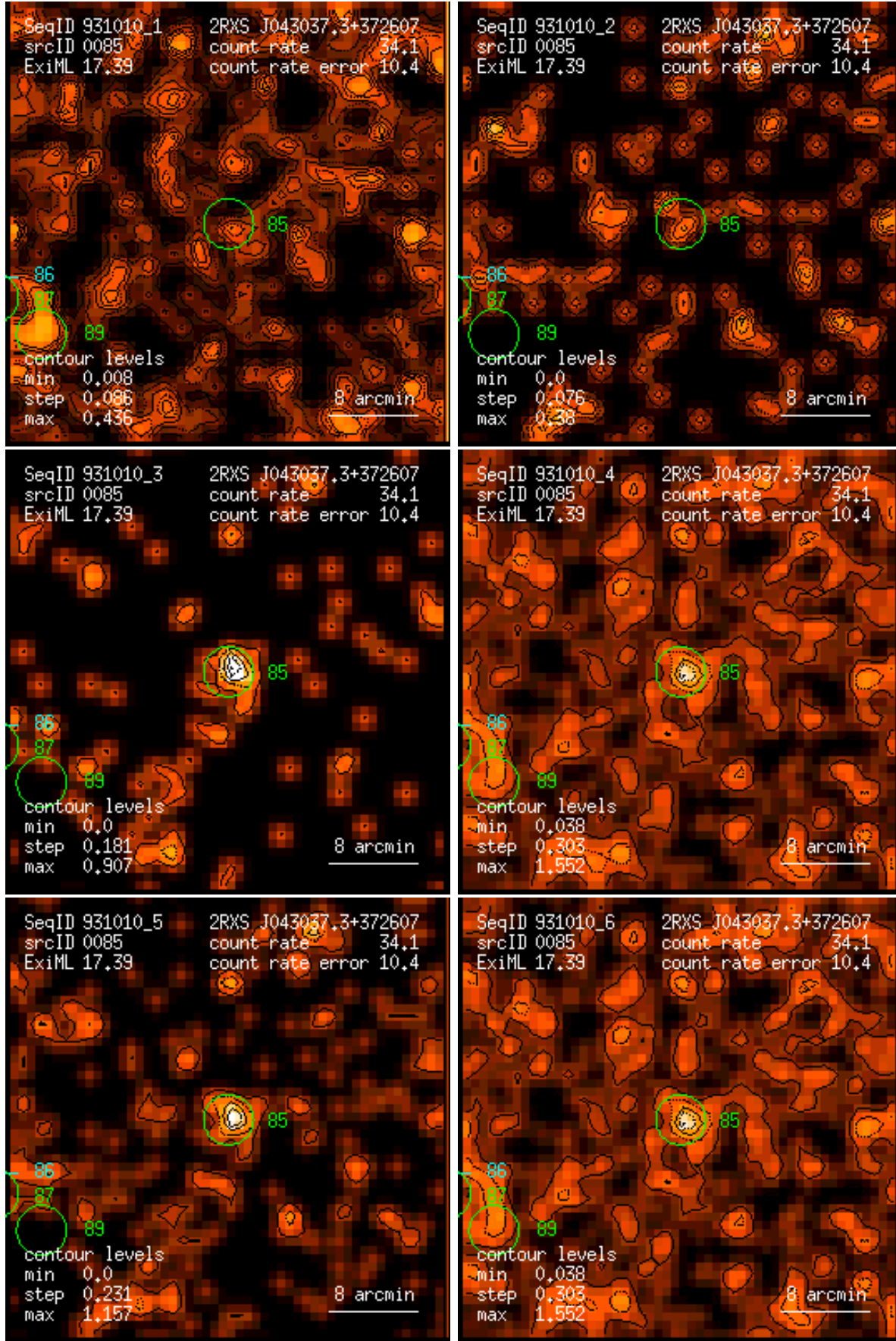
Figure 85: RASS 931010: detection 0085: band rate images, Gaussian filter: (1) PSPC channels 11 – 41, (2) 52 – 90, (3) 91 – 201, (4) 11 – 235, (5) 52 – 201, (6) 11 – 201. Broad band rates in counts/ks. Band rate contour levels in counts/ks/arcmin 2 .
