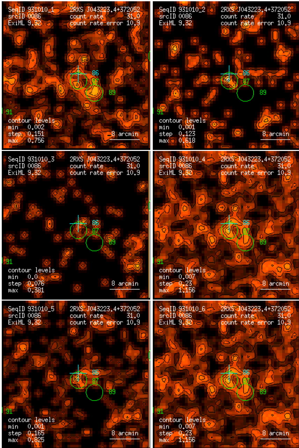
Figure 86: RASS 931010: detection 0086: band rate images, Gaussian filter: (1) PSPC channels 11 – 41, (2) 52 – 90, (3) 91 – 201, (4) 11 – 235, (5) 52 – 201, (6) 11 – 201. Broad band rates in counts/ks. Band rate contour levels in counts/ks/arcmin 2 .
