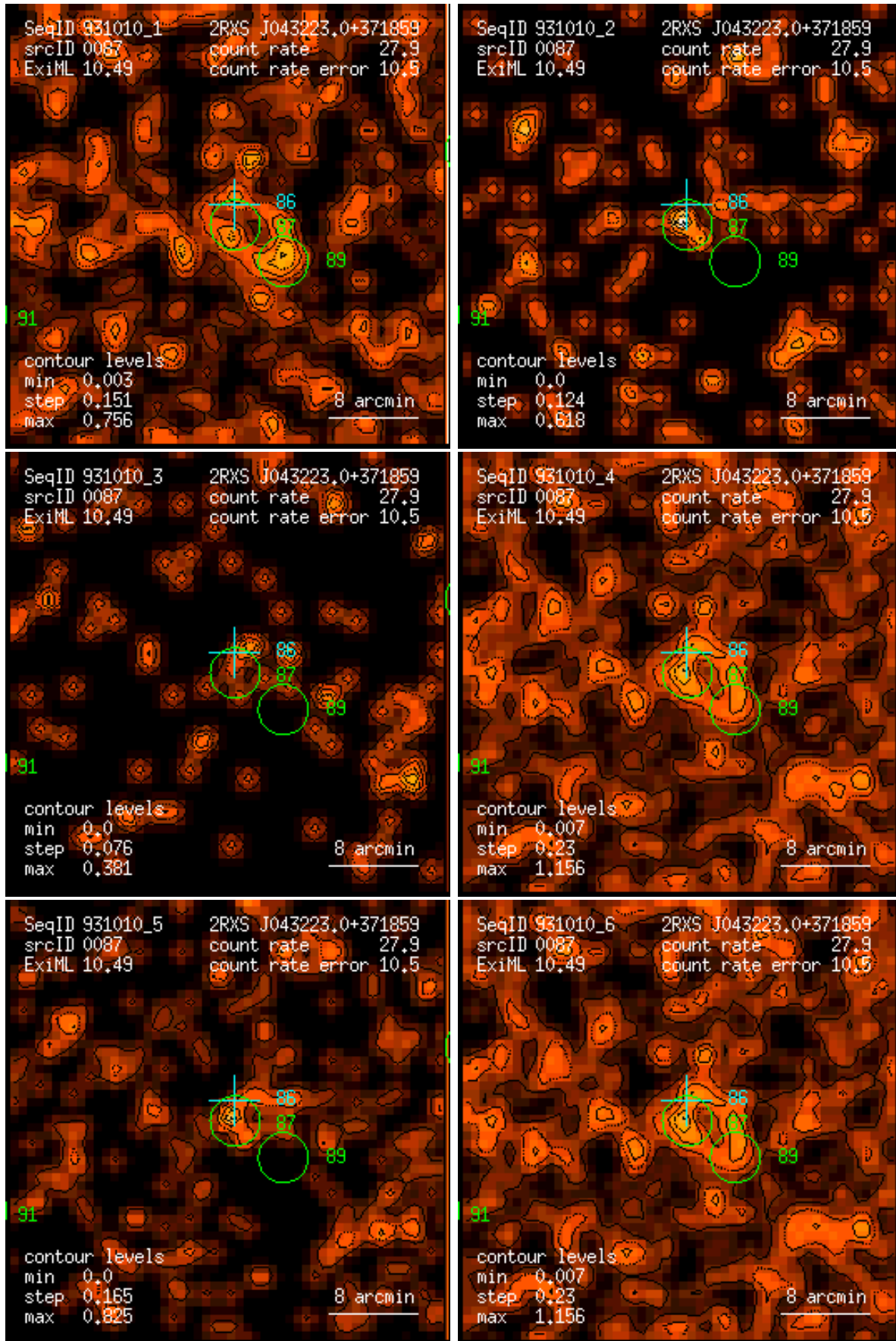
Figure 87: RASS 931010: detection 0087: band rate images, Gaussian filter: (1) PSPC channels 11 – 41, (2) 52 – 90, (3) 91 – 201, (4) 11 – 235, (5) 52 – 201, (6) 11 – 201. Broad band rates in counts/ks. Band rate contour levels in counts/ks/arcmin 2 .
