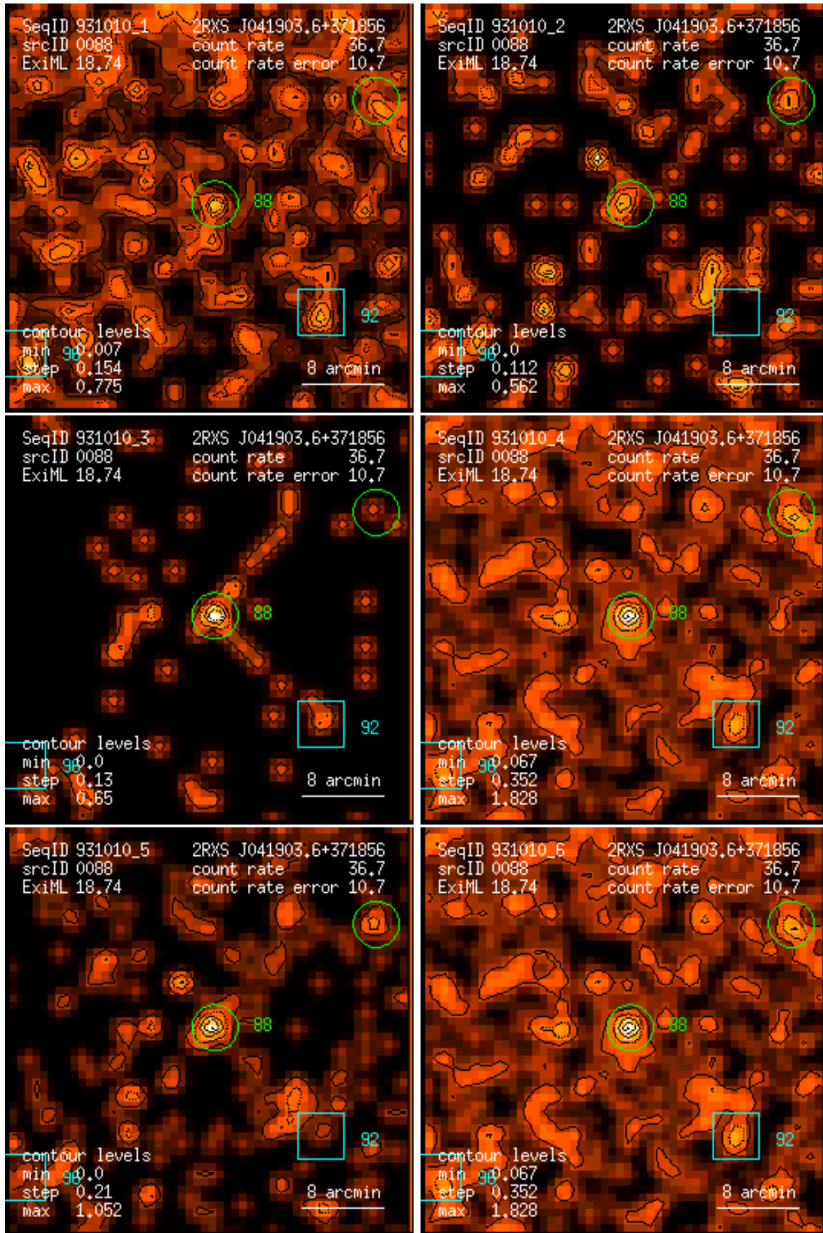
Figure 88: RASS 931010: detection 0088: band rate images, Gaussian filter: (1) PSPC channels 11 – 41, (2) 52 – 90, (3) 91 – 201, (4) 11 – 235, (5) 52 – 201, (6) 11 – 201. Broad band rates in counts/ks. Band rate contour levels in counts/ks/arcmin 2 .
