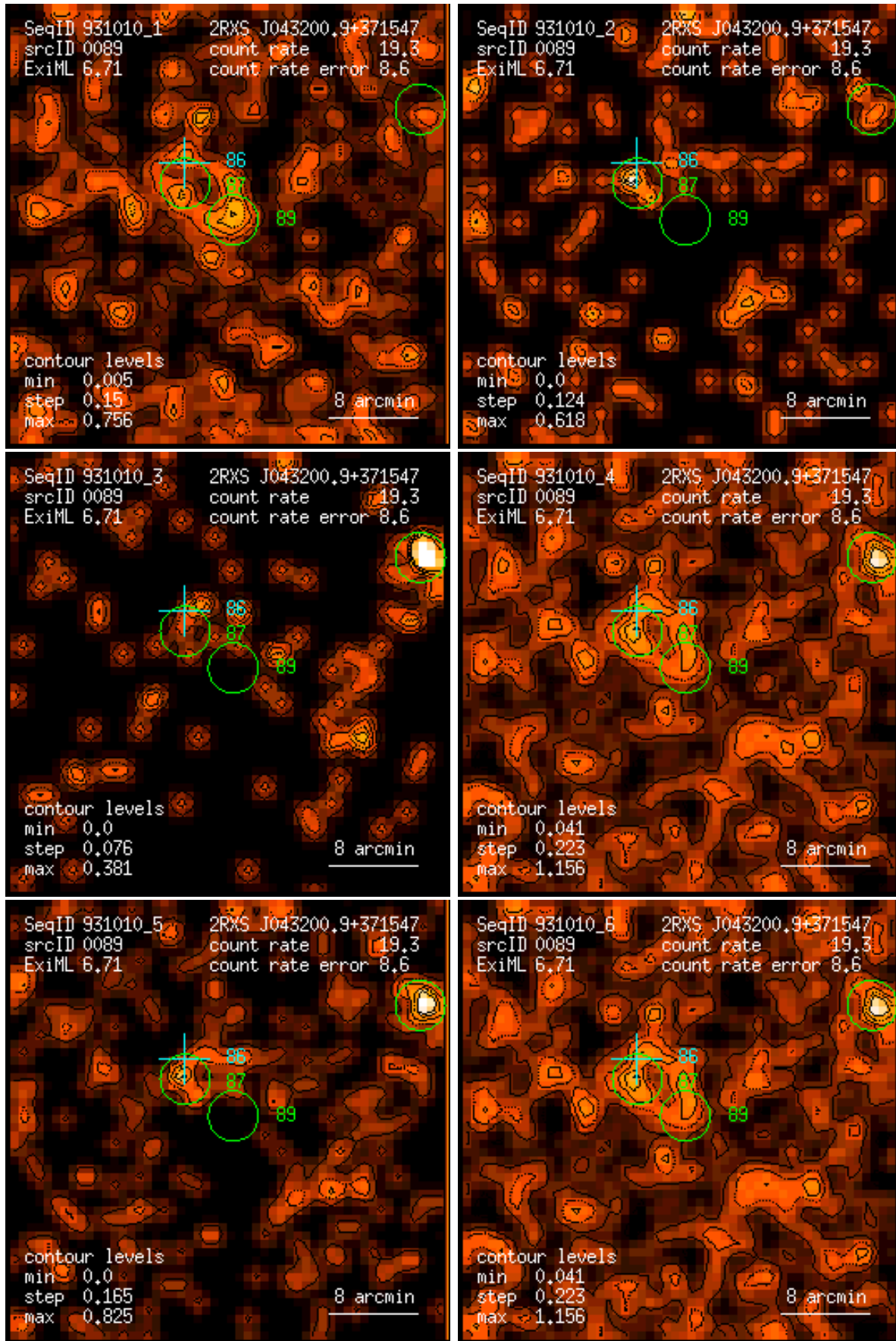
Figure 89: RASS 931010: detection 0089: band rate images, Gaussian filter: (1) PSPC channels 11 – 41, (2) 52 – 90, (3) 91 – 201, (4) 11 – 235, (5) 52 – 201, (6) 11 – 201. Broad band rates in counts/ks. Band rate contour levels in counts/ks/arcmin 2 .
