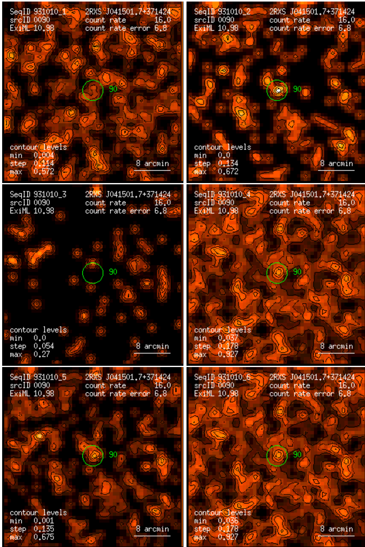
Figure 90: RASS 931010: detection 0090: band rate images, Gaussian filter: (1) PSPC channels 11 – 41, (2) 52 – 90, (3) 91 – 201, (4) 11 – 235, (5) 52 – 201, (6) 11 – 201. Broad band rates in counts/ks. Band rate contour levels in counts/ks/arcmin 2 .
