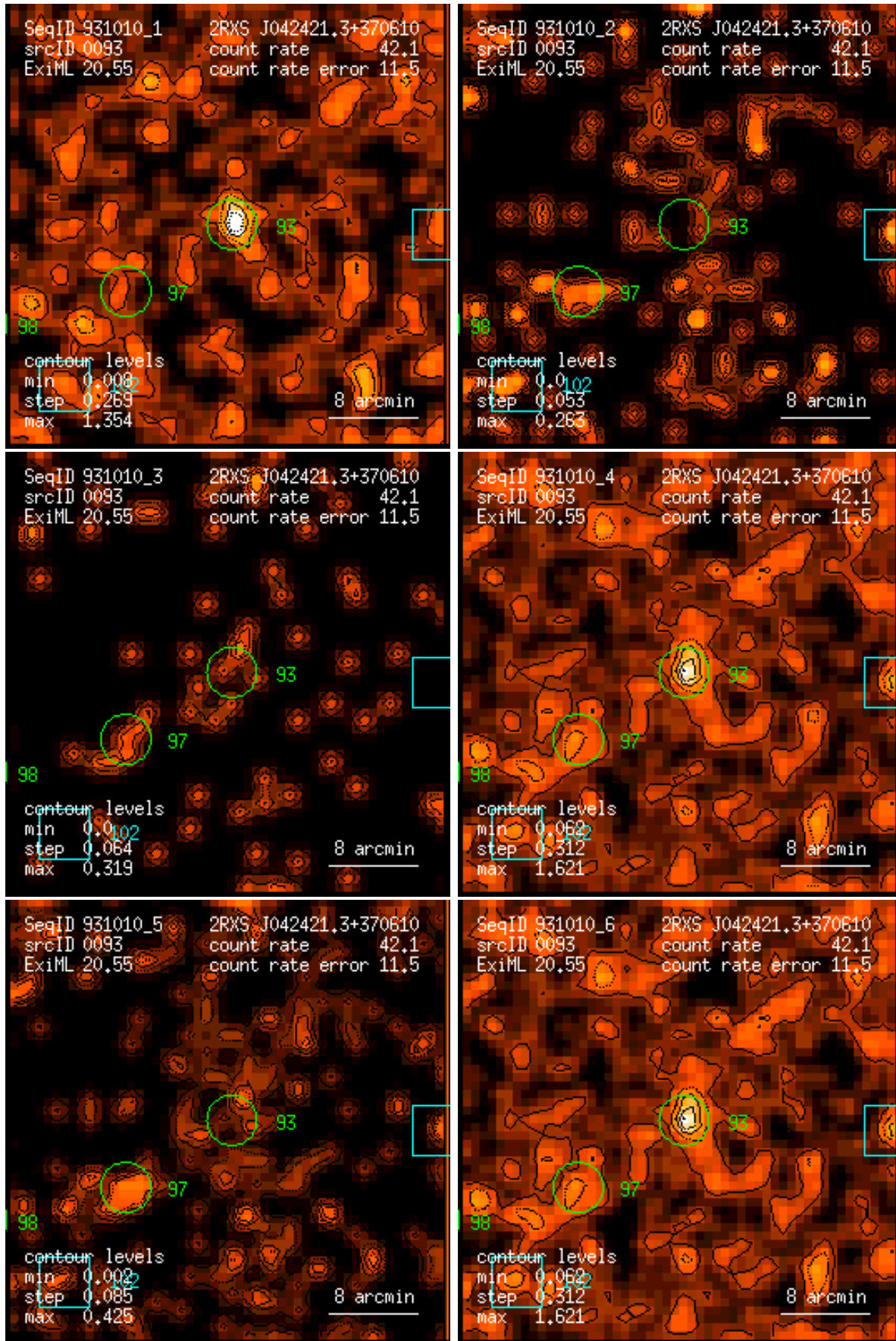
Figure 93: RASS 931010: detection 0093: band rate images, Gaussian filter: (1) PSPC channels 11 – 41, (2) 52 – 90, (3) 91 – 201, (4) 11 – 235, (5) 52 – 201, (6) 11 – 201. Broad band rates in counts/ks. Band rate contour levels in counts/ks/arcmin 2 .
