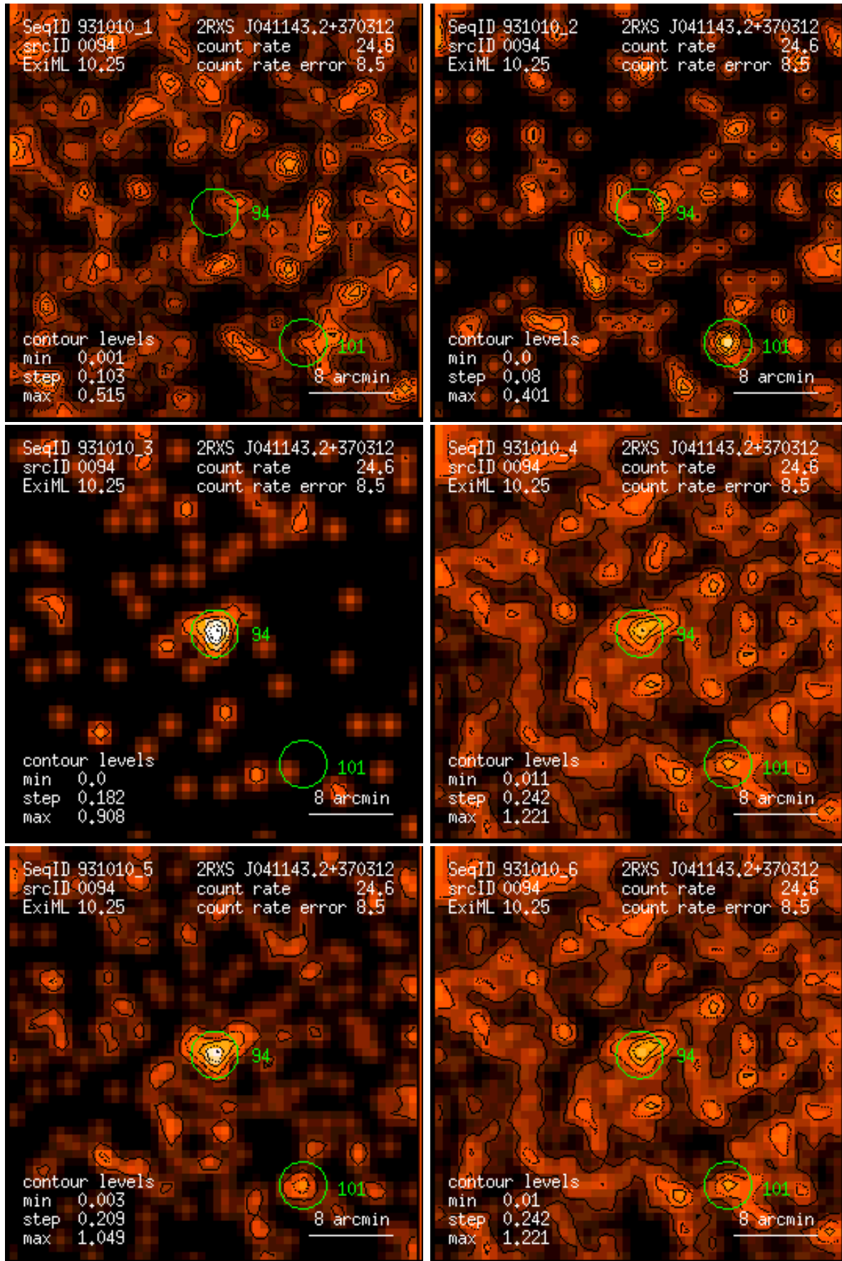
Figure 94: RASS 931010: detection 0094: band rate images, Gaussian filter: (1) PSPC channels 11 – 41, (2) 52 – 90, (3) 91 – 201, (4) 11 – 235, (5) 52 – 201, (6) 11 – 201. Broad band rates in counts/ks. Band rate contour levels in counts/ks/arcmin 2 .
