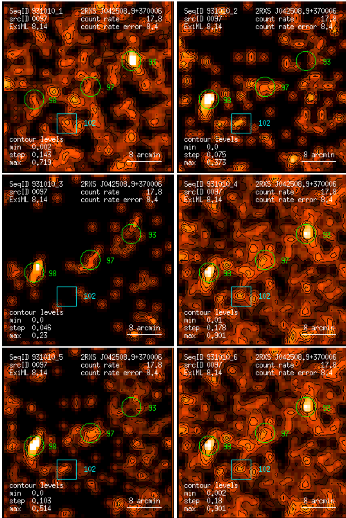
Figure 97: RASS 931010: detection 0097: band rate images, Gaussian filter: (1) PSPC channels 11 – 41, (2) 52 – 90, (3) 91 – 201, (4) 11 – 235, (5) 52 – 201, (6) 11 – 201. Broad band rates in counts/ks. Band rate contour levels in counts/ks/arcmin 2 .
