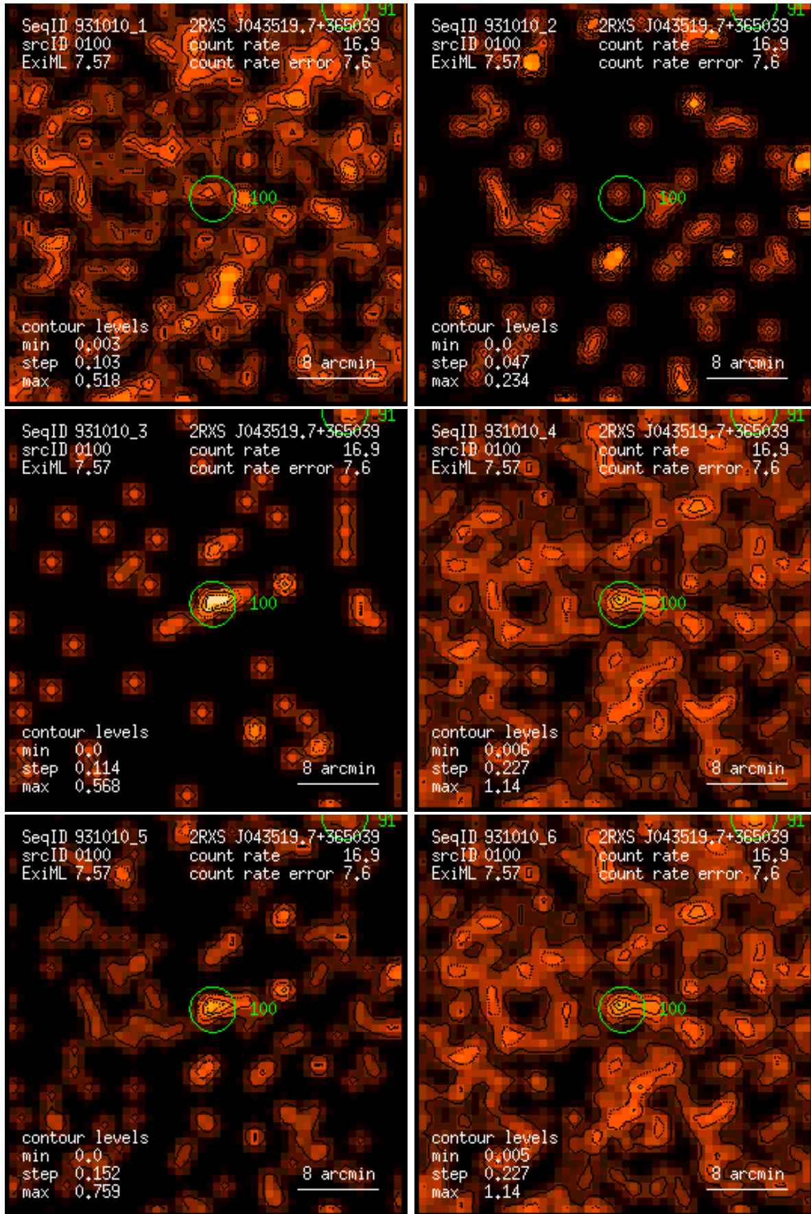
Figure 100: RASS 931010: detection 0100: band rate images, Gaussian filter: (1) PSPC channels 11 – 41, (2) 52 – 90, (3) 91 – 201, (4) 11 – 235, (5) 52 – 201, (6) 11 – 201. Broad band rates in counts/ks. Band rate contour levels in counts/ks/arcmin 2 .
