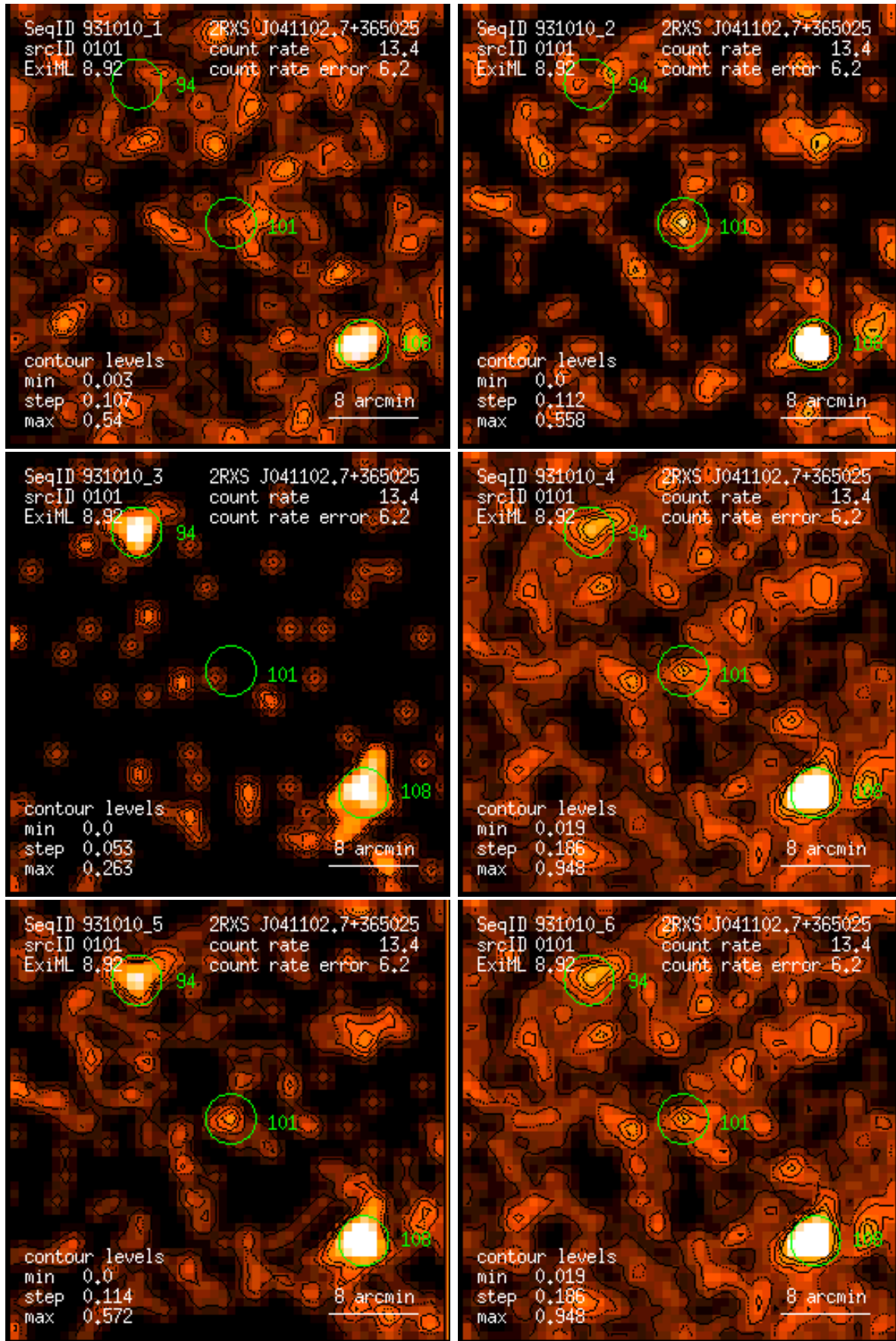
Figure 101: RASS 931010: detection 0101: band rate images, Gaussian filter: (1) PSPC channels 11 – 41, (2) 52 – 90, (3) 91 – 201, (4) 11 – 235, (5) 52 – 201, (6) 11 – 201. Broad band rates in counts/ks. Band rate contour levels in counts/ks/arcmin 2 .
