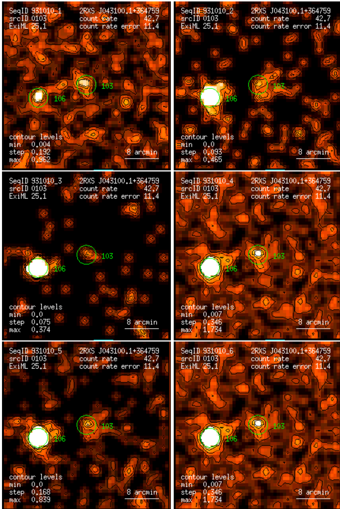
Figure 103: RASS 931010: detection 0103: band rate images, Gaussian filter: (1) PSPC channels 11 – 41, (2) 52 – 90, (3) 91 – 201, (4) 11 – 235, (5) 52 – 201, (6) 11 – 201. Broad band rates in counts/ks. Band rate contour levels in counts/ks/arcmin 2 .
