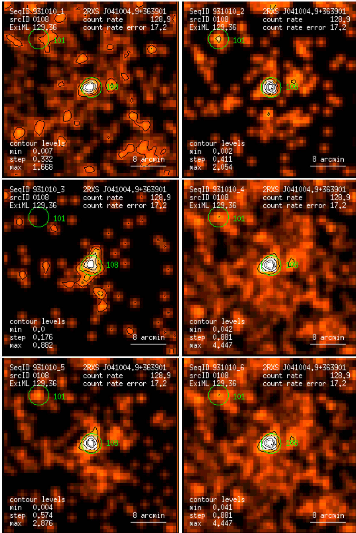
Figure 108: RASS 931010: detection 0108: band rate images, Gaussian filter: (1) PSPC channels 11 – 41, (2) 52 – 90, (3) 91 – 201, (4) 11 – 235, (5) 52 – 201, (6) 11 – 201. Broad band rates in counts/ks. Band rate contour levels in counts/ks/arcmin 2 .
