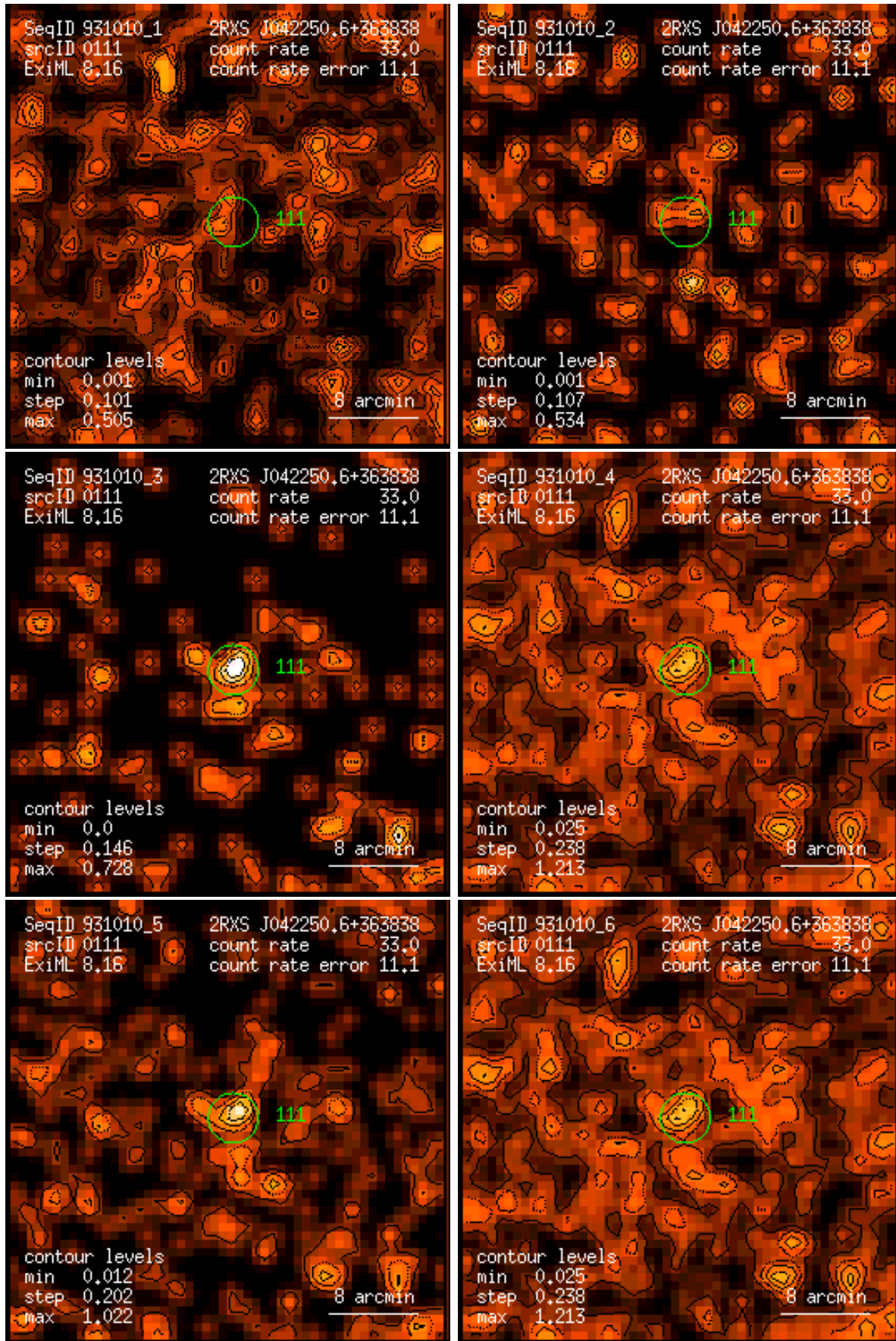
Figure 111: RASS 931010: detection 0111: band rate images, Gaussian filter: (1) PSPC channels 11 – 41, (2) 52 – 90, (3) 91 – 201, (4) 11 – 235, (5) 52 – 201, (6) 11 – 201. Broad band rates in counts/ks. Band rate contour levels in counts/ks/arcmin 2 .
