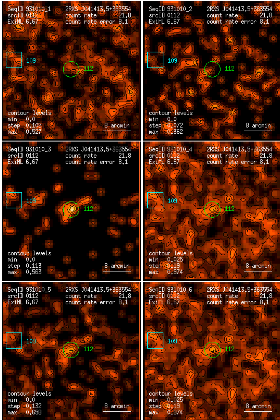
Figure 112: RASS 931010: detection 0112: band rate images, Gaussian filter: (1) PSPC channels 11 – 41, (2) 52 – 90, (3) 91 – 201, (4) 11 – 235, (5) 52 – 201, (6) 11 – 201. Broad band rates in counts/ks. Band rate contour levels in counts/ks/arcmin 2 .
