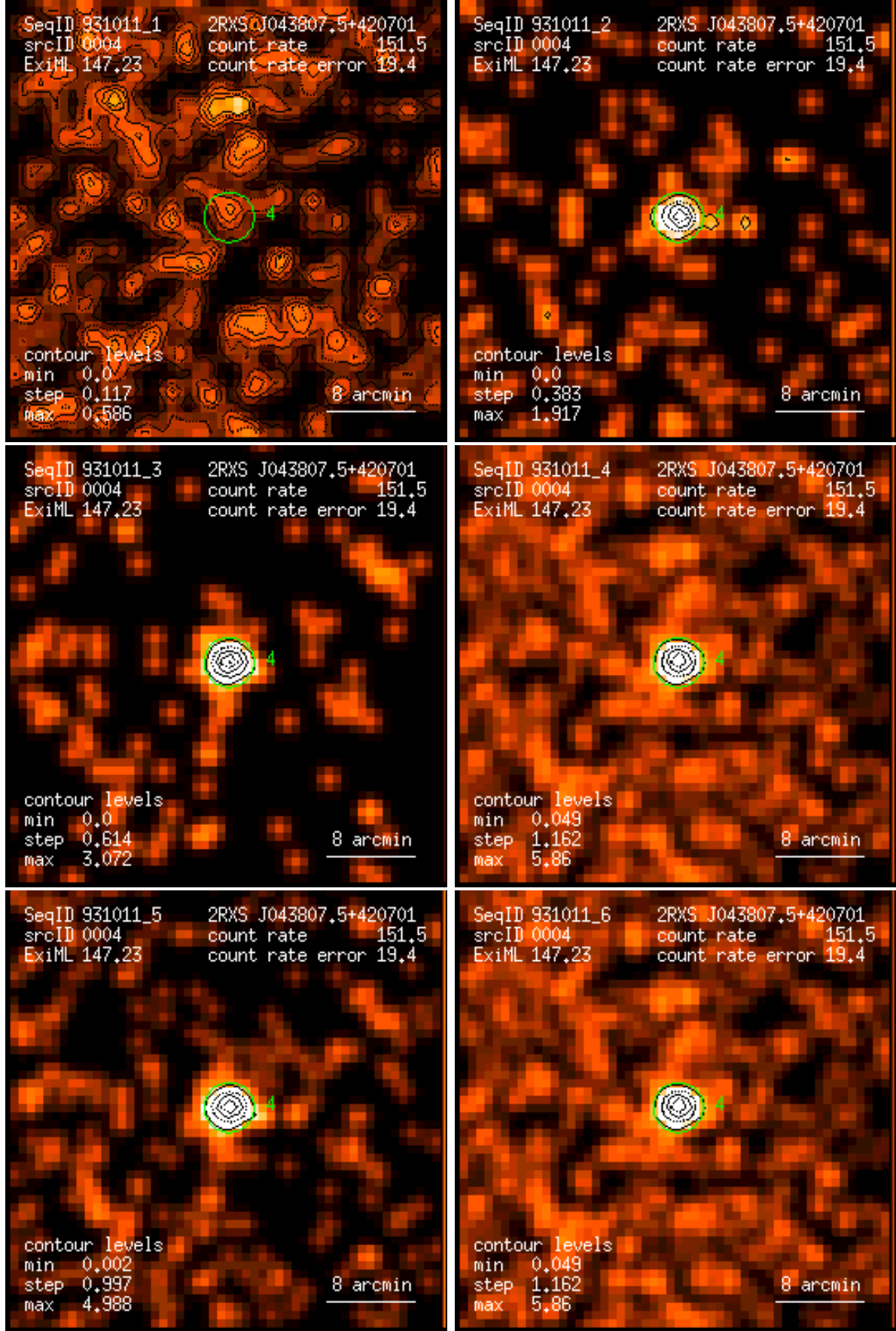
Figure 4: RASS 931011: detection 0004: band rate images, Gaussian filter: (1) PSPC channels 11 – 41, (2) 52 – 90, (3) 91 – 201, (4) 11 – 235, (5) 52 – 201, (6) 11 – 201. Broad band rates in counts/ks. Band rate contour levels in counts/ks/arcmin 2 .
