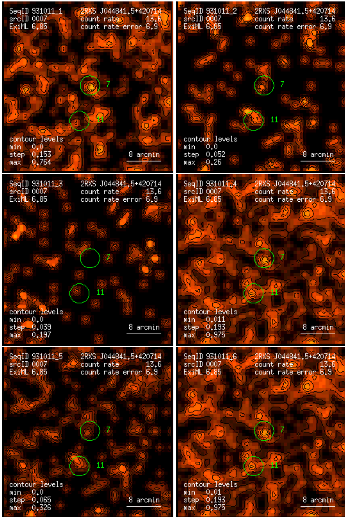
Figure 7: RASS 931011: detection 0007: band rate images, Gaussian filter: (1) PSPC channels 11 – 41, (2) 52 – 90, (3) 91 – 201, (4) 11 – 235, (5) 52 – 201, (6) 11 – 201. Broad band rates in counts/ks. Band rate contour levels in counts/ks/arcmin 2 .
