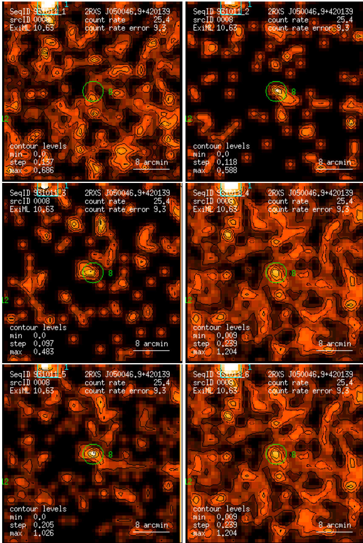
Figure 8: RASS 931011: detection 0008: band rate images, Gaussian filter: (1) PSPC channels 11 – 41, (2) 52 – 90, (3) 91 – 201, (4) 11 – 235, (5) 52 – 201, (6) 11 – 201. Broad band rates in counts/ks. Band rate contour levels in counts/ks/arcmin 2 .
