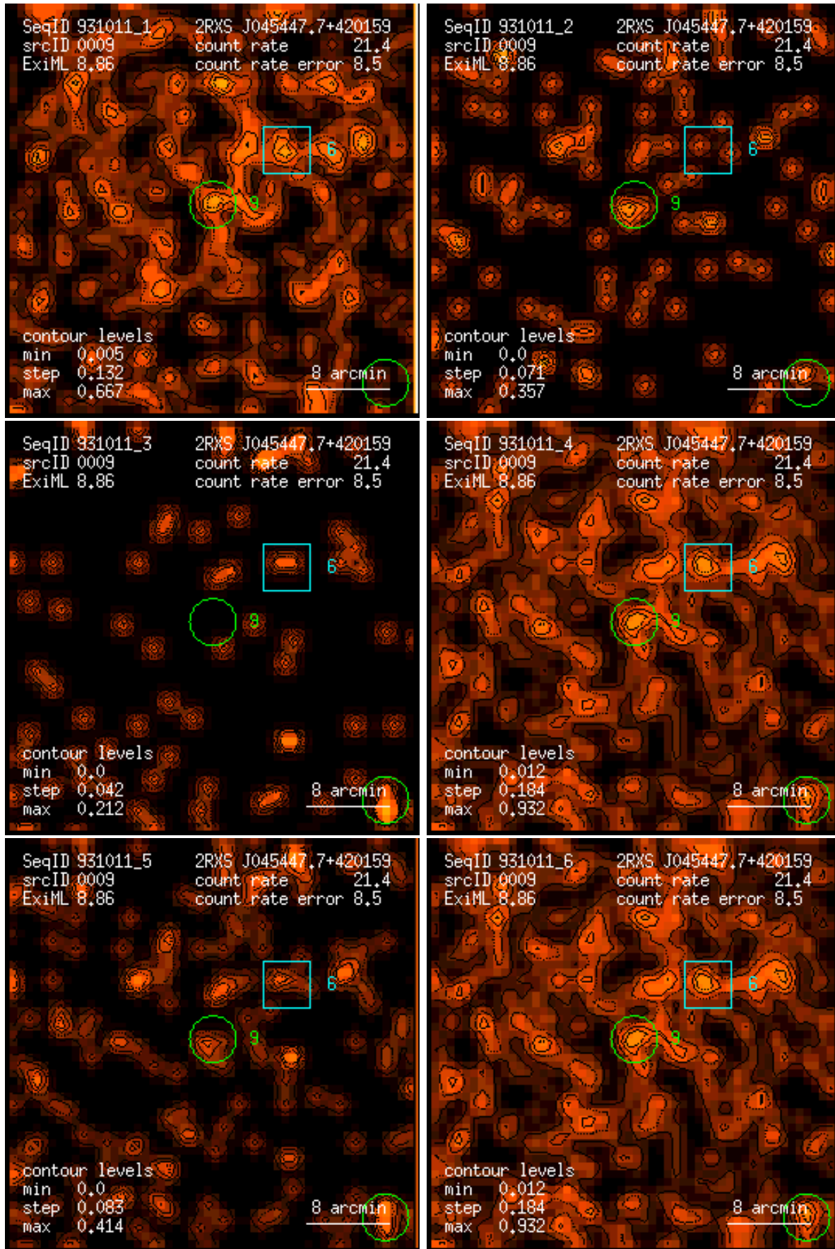
Figure 9: RASS 931011: detection 0009: band rate images, Gaussian filter: (1) PSPC channels 11 – 41, (2) 52 – 90, (3) 91 – 201, (4) 11 – 235, (5) 52 – 201, (6) 11 – 201. Broad band rates in counts/ks. Band rate contour levels in counts/ks/arcmin 2 .
