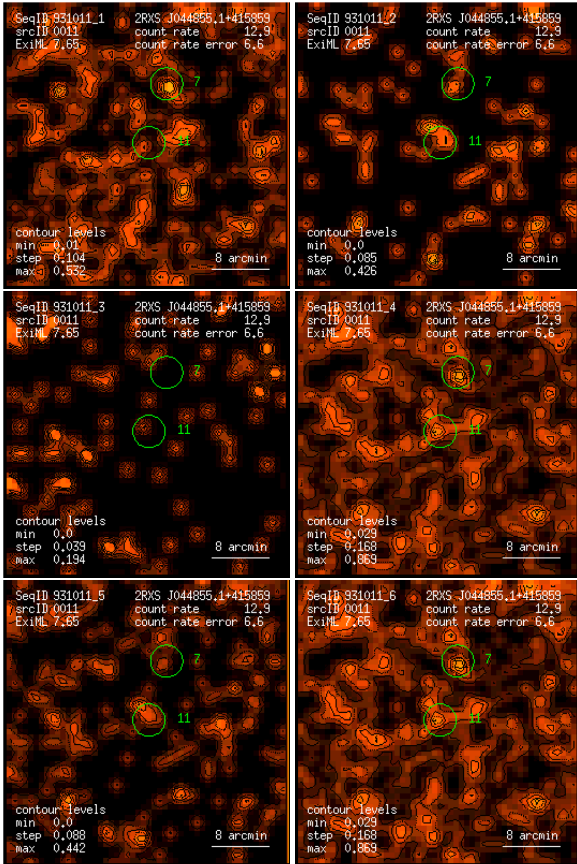
Figure 11: RASS 931011: detection 0011: band rate images, Gaussian filter: (1) PSPC channels 11 – 41, (2) 52 – 90, (3) 91 – 201, (4) 11 – 235, (5) 52 – 201, (6) 11 – 201. Broad band rates in counts/ks. Band rate contour levels in counts/ks/arcmin 2 .
