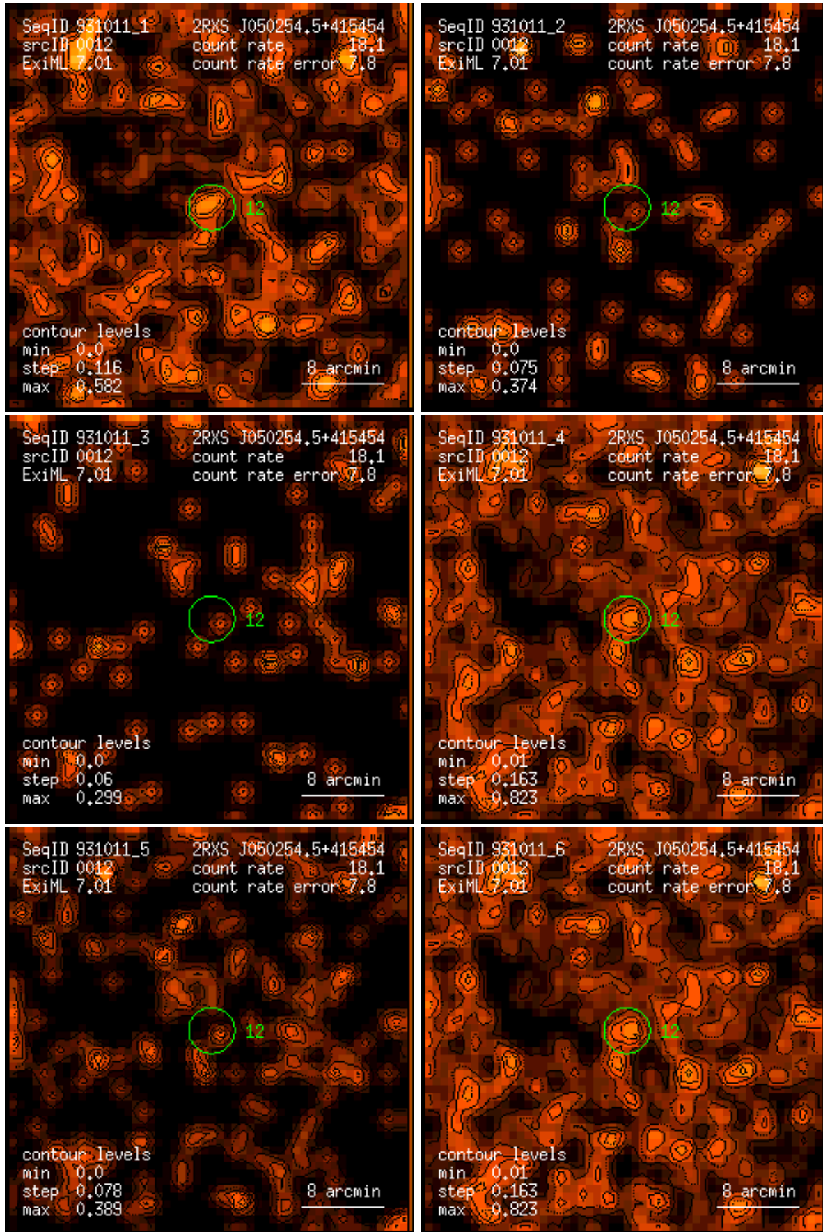
Figure 12: RASS 931011: detection 0012: band rate images, Gaussian filter: (1) PSPC channels 11 – 41, (2) 52 – 90, (3) 91 – 201, (4) 11 – 235, (5) 52 – 201, (6) 11 – 201. Broad band rates in counts/ks. Band rate contour levels in counts/ks/arcmin 2 .
