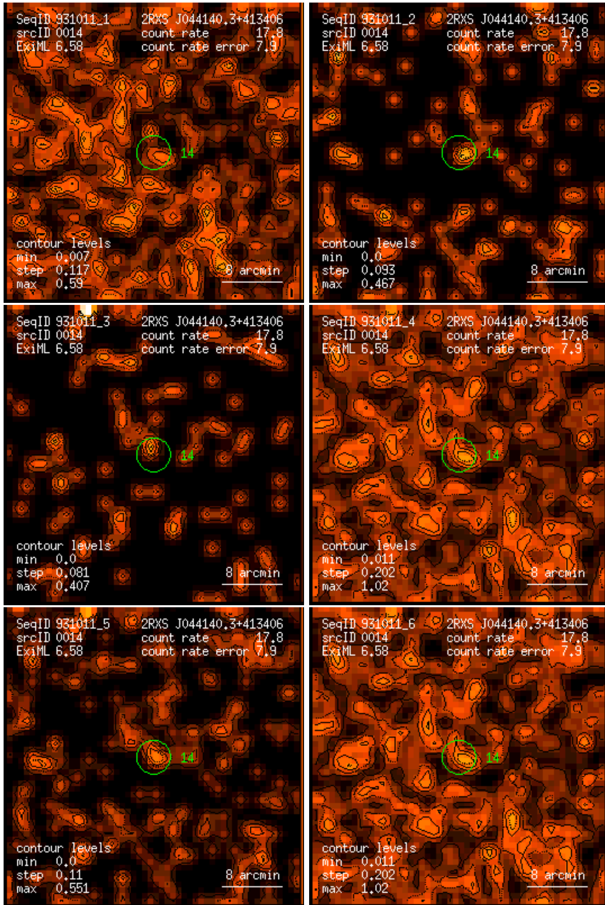
Figure 14: RASS 931011: detection 0014: band rate images, Gaussian filter: (1) PSPC channels 11 – 41, (2) 52 – 90, (3) 91 – 201, (4) 11 – 235, (5) 52 – 201, (6) 11 – 201. Broad band rates in counts/ks. Band rate contour levels in counts/ks/arcmin 2 .
