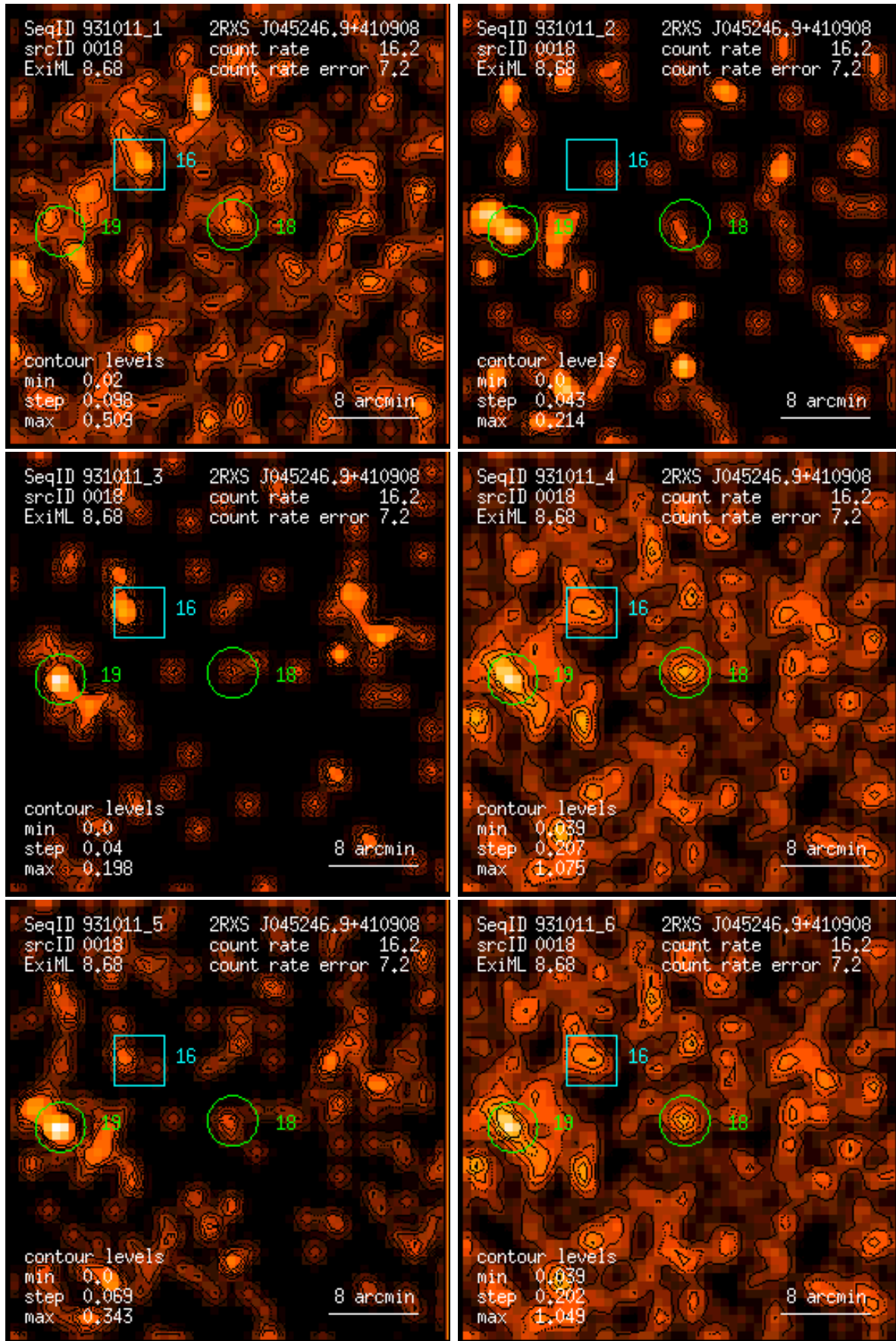
Figure 18: RASS 931011: detection 0018: band rate images, Gaussian filter: (1) PSPC channels 11 – 41, (2) 52 – 90, (3) 91 – 201, (4) 11 – 235, (5) 52 – 201, (6) 11 – 201. Broad band rates in counts/ks. Band rate contour levels in counts/ks/arcmin 2 .
