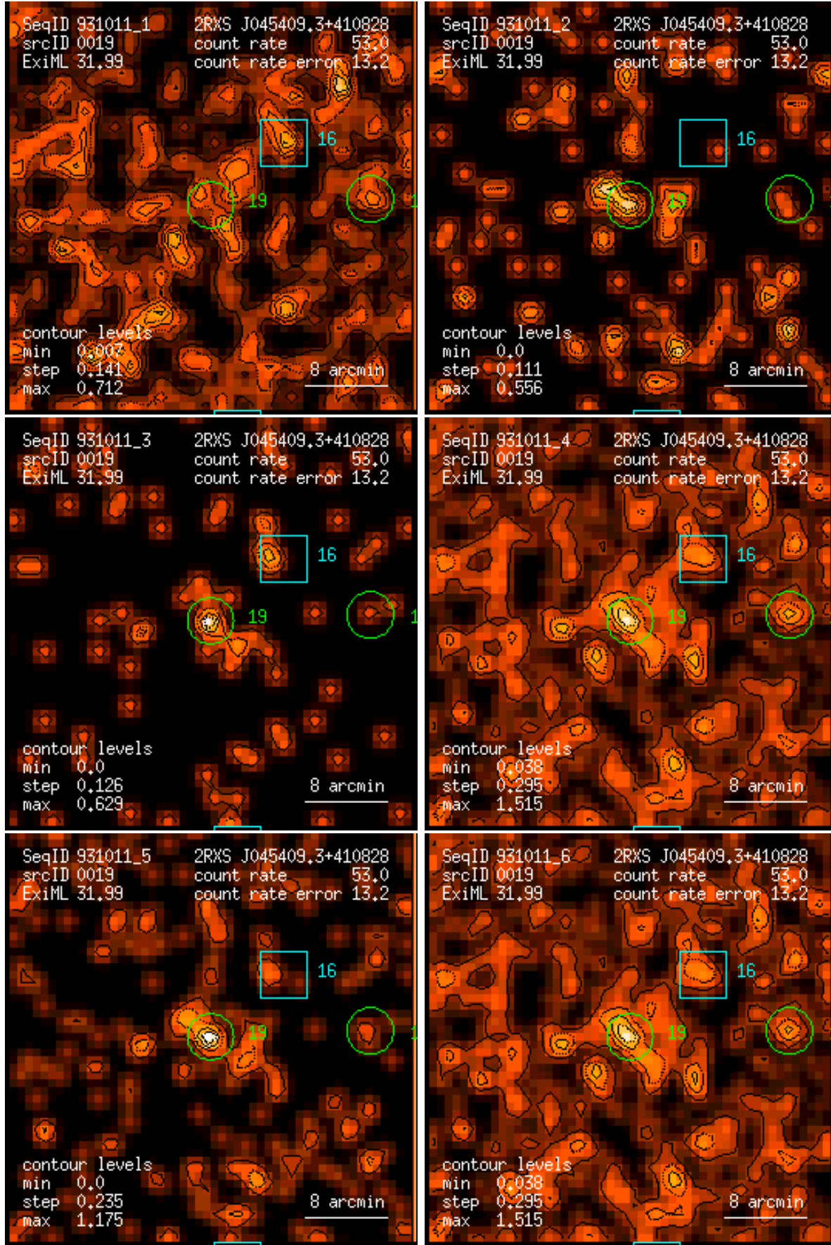
Figure 19: RASS 931011: detection 0019: band rate images, Gaussian filter: (1) PSPC channels 11 – 41, (2) 52 – 90, (3) 91 – 201, (4) 11 – 235, (5) 52 – 201, (6) 11 – 201. Broad band rates in counts/ks. Band rate contour levels in counts/ks/arcmin 2 .
