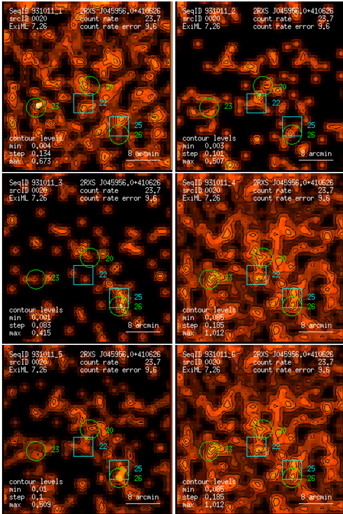
Figure 20: RASS 931011: detection 0020: band rate images, Gaussian filter: (1) PSPC channels 11 – 41, (2) 52 – 90, (3) 91 – 201, (4) 11 – 235, (5) 52 – 201, (6) 11 – 201. Broad band rates in counts/ks. Band rate contour levels in counts/ks/arcmin 2 .
