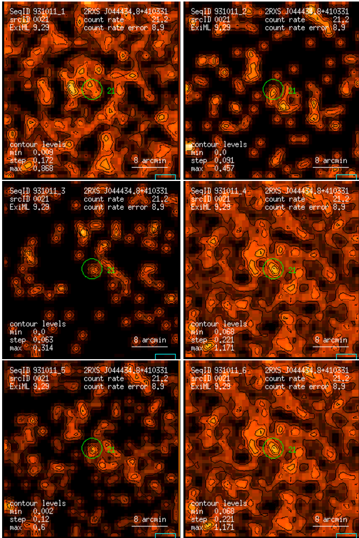
Figure 21: RASS 931011: detection 0021: band rate images, Gaussian filter: (1) PSPC channels 11 – 41, (2) 52 – 90, (3) 91 – 201, (4) 11 – 235, (5) 52 – 201, (6) 11 – 201. Broad band rates in counts/ks. Band rate contour levels in counts/ks/arcmin 2 .
