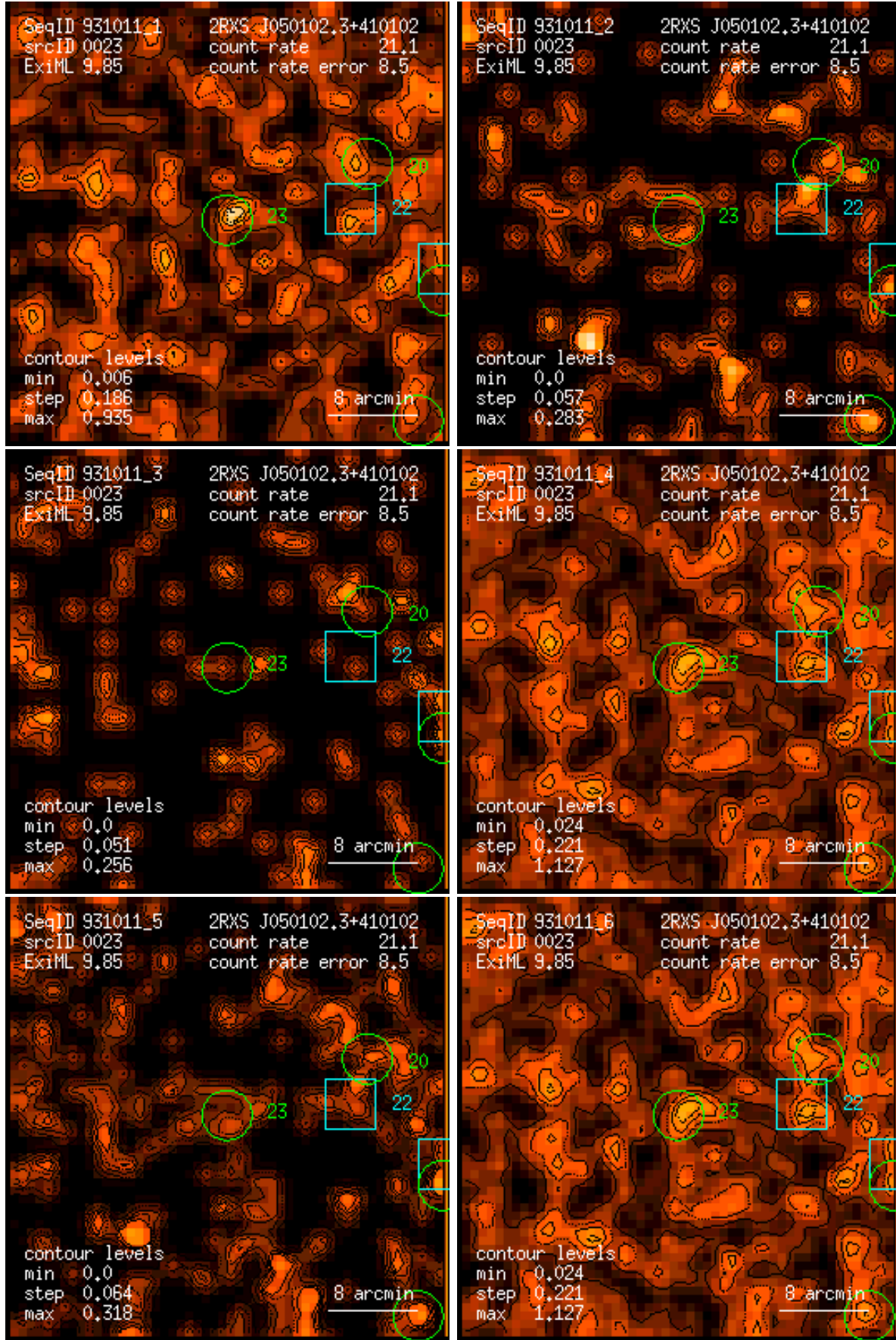
Figure 23: RASS 931011: detection 0023: band rate images, Gaussian filter: (1) PSPC channels 11 – 41, (2) 52 – 90, (3) 91 – 201, (4) 11 – 235, (5) 52 – 201, (6) 11 – 201. Broad band rates in counts/ks. Band rate contour levels in counts/ks/arcmin 2 .
