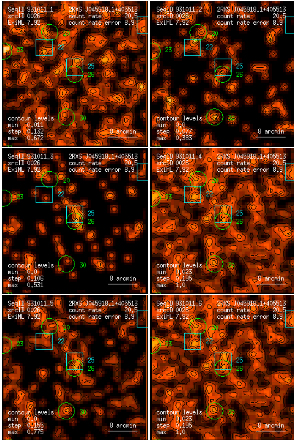
Figure 26: RASS 931011: detection 0026: band rate images, Gaussian filter: (1) PSPC channels 11 – 41, (2) 52 – 90, (3) 91 – 201, (4) 11 – 235, (5) 52 – 201, (6) 11 – 201. Broad band rates in counts/ks. Band rate contour levels in counts/ks/arcmin 2 .
