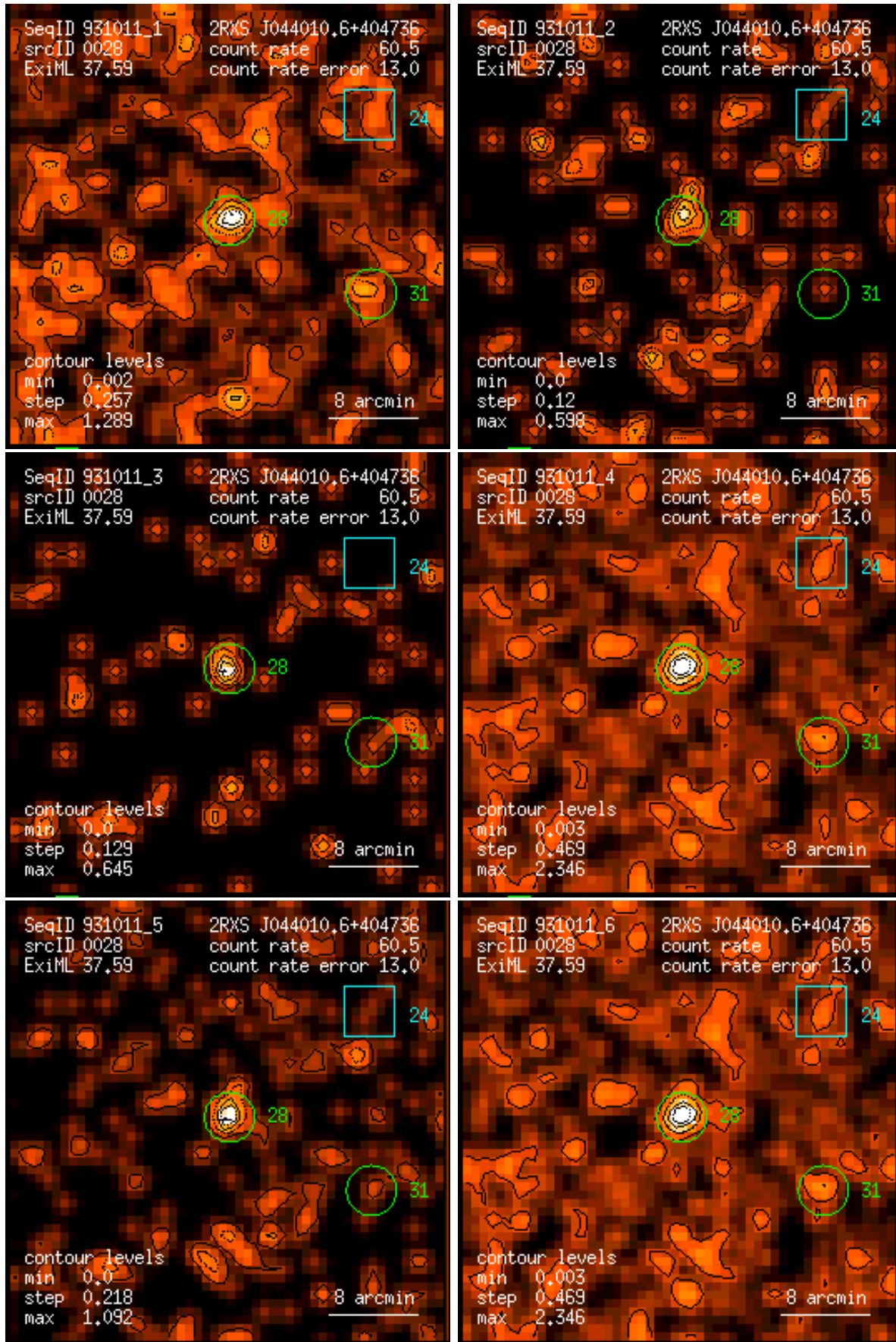
Figure 28: RASS 931011: detection 0028: band rate images, Gaussian filter: (1) PSPC channels 11 – 41, (2) 52 – 90, (3) 91 – 201, (4) 11 – 235, (5) 52 – 201, (6) 11 – 201. Broad band rates in counts/ks. Band rate contour levels in counts/ks/arcmin 2 .
