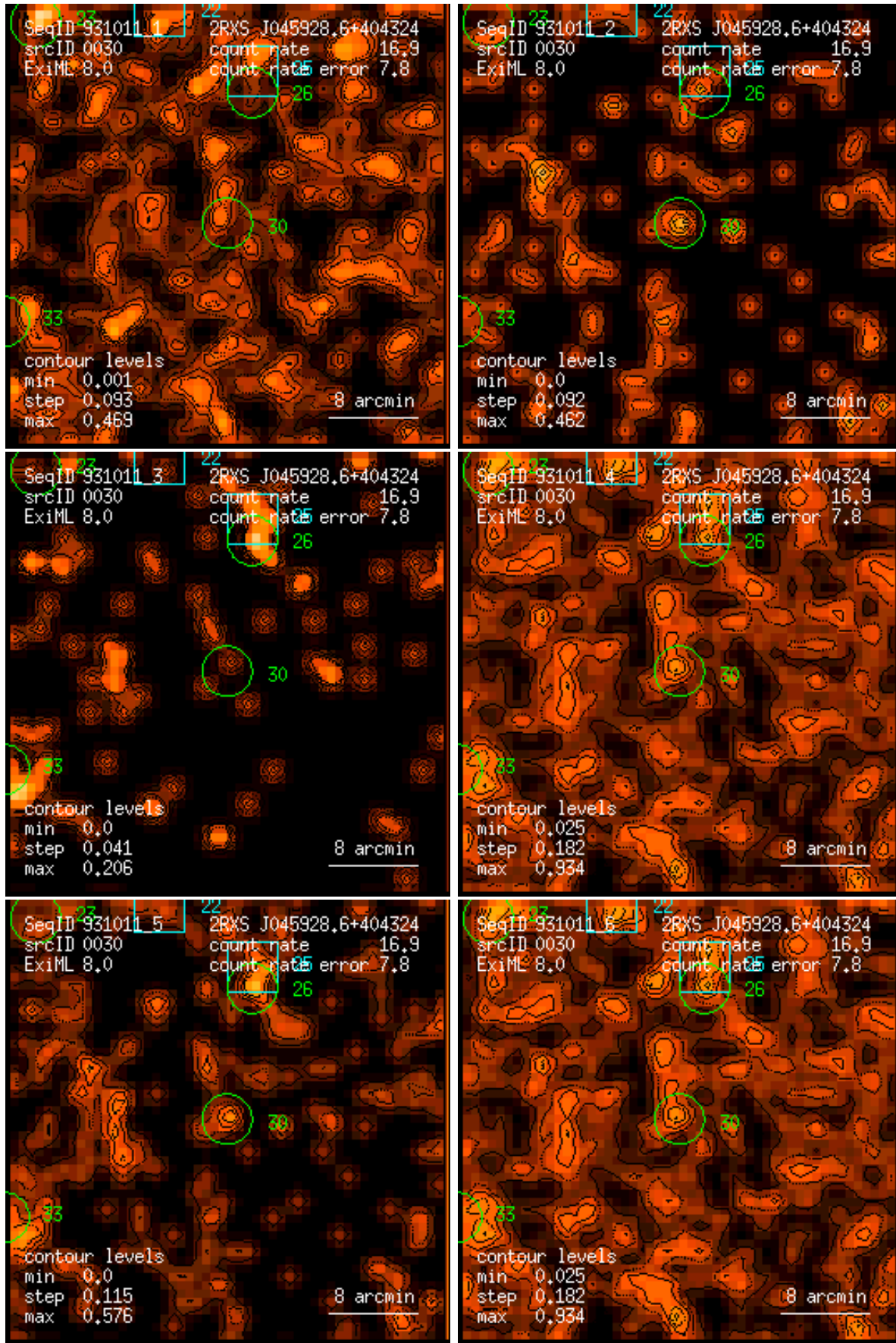
Figure 30: RASS 931011: detection 0030: band rate images, Gaussian filter: (1) PSPC channels 11 – 41, (2) 52 – 90, (3) 91 – 201, (4) 11 – 235, (5) 52 – 201, (6) 11 – 201. Broad band rates in counts/ks. Band rate contour levels in counts/ks/arcmin 2 .
