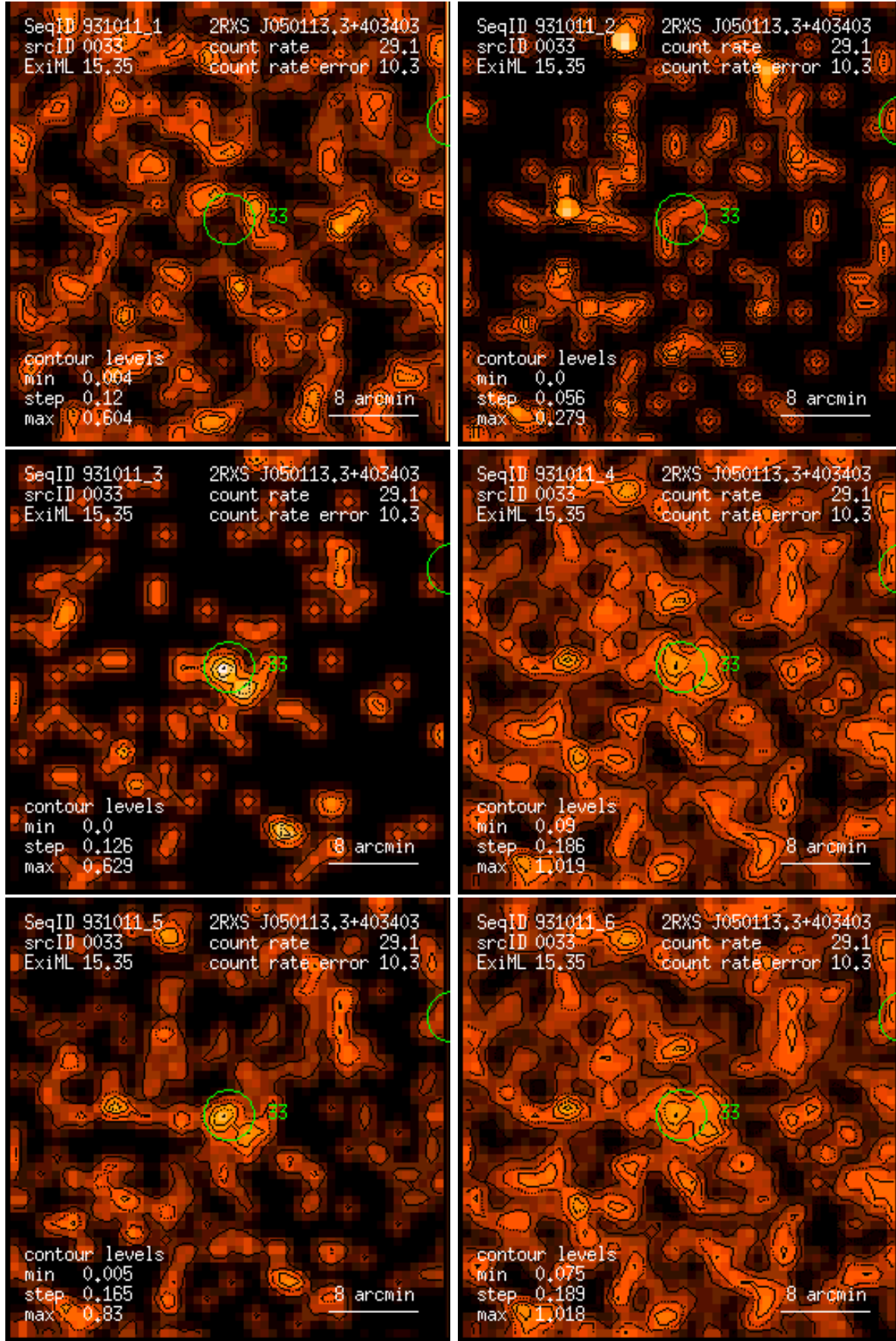
Figure 33: RASS 931011: detection 0033: band rate images, Gaussian filter: (1) PSPC channels 11 – 41, (2) 52 – 90, (3) 91 – 201, (4) 11 – 235, (5) 52 – 201, (6) 11 – 201. Broad band rates in counts/ks. Band rate contour levels in counts/ks/arcmin 2 .
