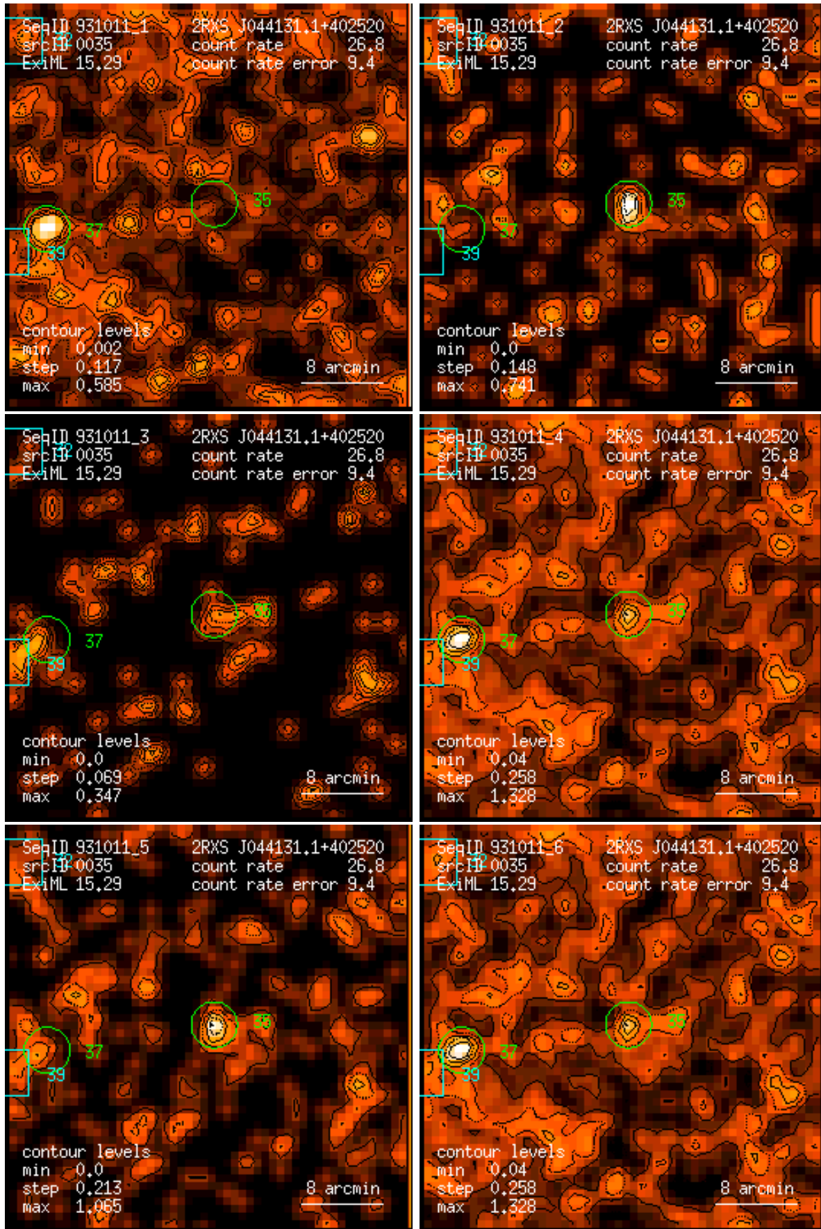
Figure 35: RASS 931011: detection 0035: band rate images, Gaussian filter: (1) PSPC channels 11 – 41, (2) 52 – 90, (3) 91 – 201, (4) 11 – 235, (5) 52 – 201, (6) 11 – 201. Broad band rates in counts/ks. Band rate contour levels in counts/ks/arcmin 2 .
