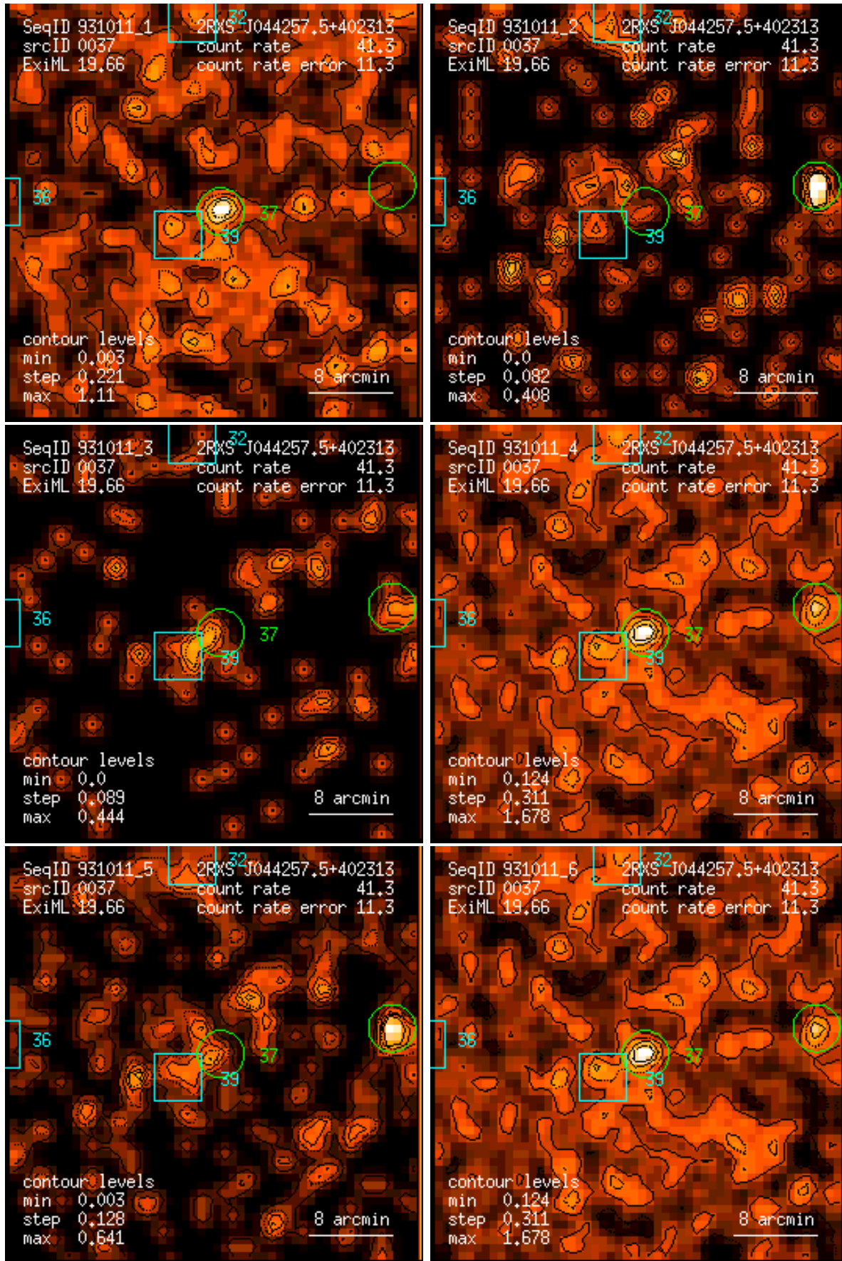
Figure 37: RASS 931011: detection 0037: band rate images, Gaussian filter: (1) PSPC channels 11 – 41, (2) 52 – 90, (3) 91 – 201, (4) 11 – 235, (5) 52 – 201, (6) 11 – 201. Broad band rates in counts/ks. Band rate contour levels in counts/ks/arcmin 2 .
