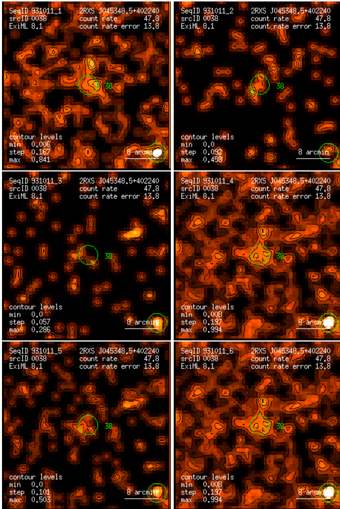
Figure 38: RASS 931011: detection 0038: band rate images, Gaussian filter: (1) PSPC channels 11 – 41, (2) 52 – 90, (3) 91 – 201, (4) 11 – 235, (5) 52 – 201, (6) 11 – 201. Broad band rates in counts/ks. Band rate contour levels in counts/ks/arcmin 2 .
