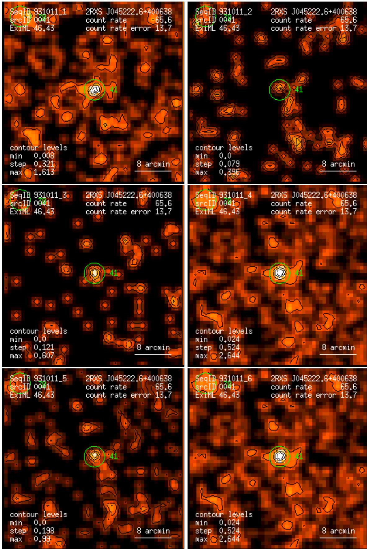
Figure 41: RASS 931011: detection 0041: band rate images, Gaussian filter: (1) PSPC channels 11 – 41, (2) 52 – 90, (3) 91 – 201, (4) 11 – 235, (5) 52 – 201, (6) 11 – 201. Broad band rates in counts/ks. Band rate contour levels in counts/ks/arcmin 2 .
