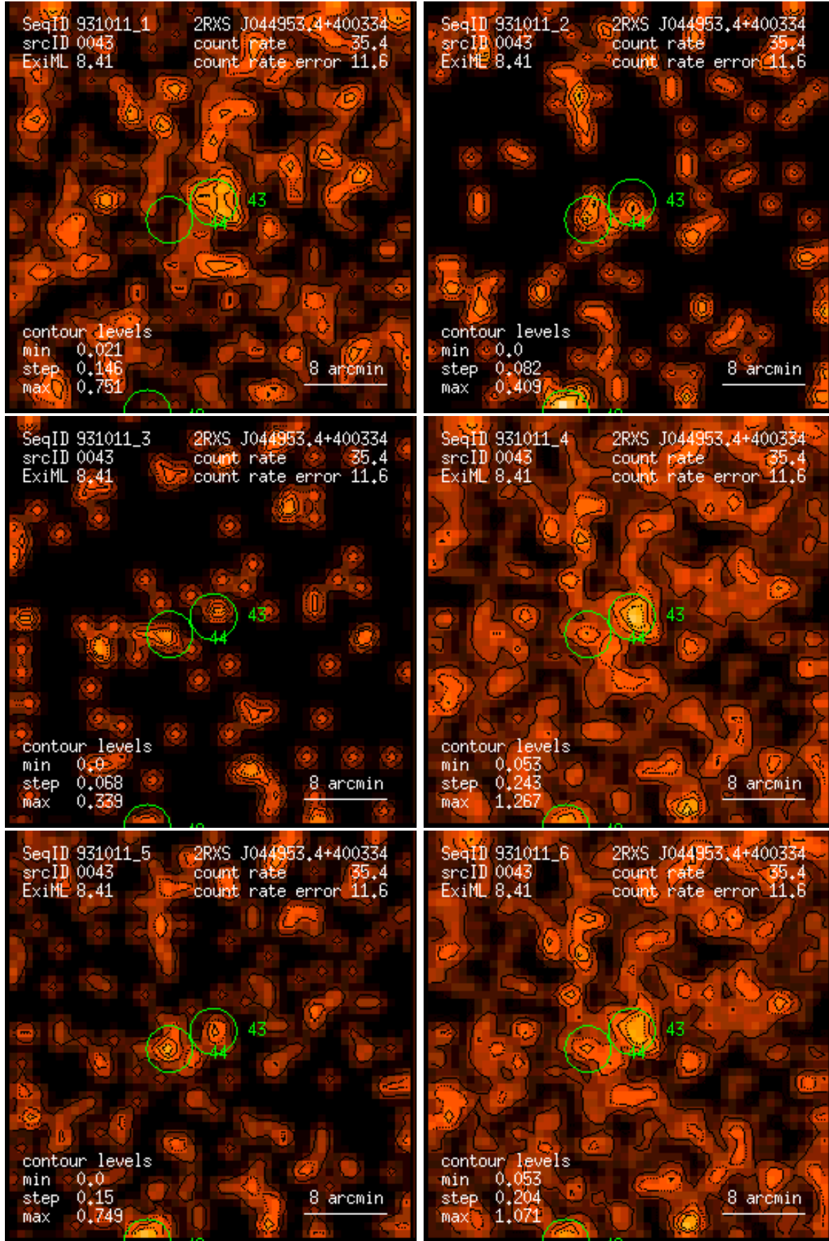
Figure 43: RASS 931011: detection 0043: band rate images, Gaussian filter: (1) PSPC channels 11 – 41, (2) 52 – 90, (3) 91 – 201, (4) 11 – 235, (5) 52 – 201, (6) 11 – 201. Broad band rates in counts/ks. Band rate contour levels in counts/ks/arcmin 2 .
