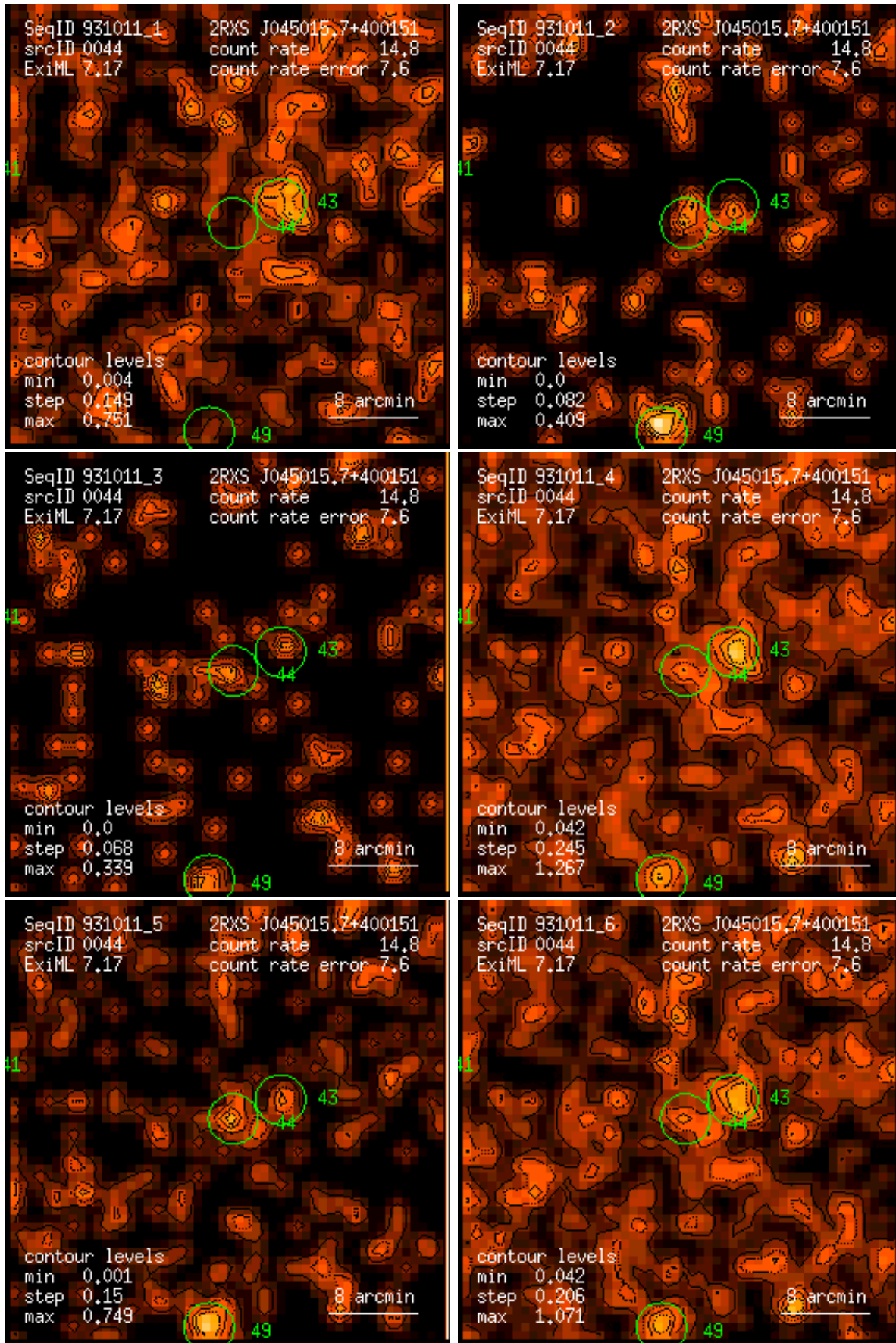
Figure 44: RASS 931011: detection 0044: band rate images, Gaussian filter: (1) PSPC channels 11 – 41, (2) 52 – 90, (3) 91 – 201, (4) 11 – 235, (5) 52 – 201, (6) 11 – 201. Broad band rates in counts/ks. Band rate contour levels in counts/ks/arcmin 2 .
