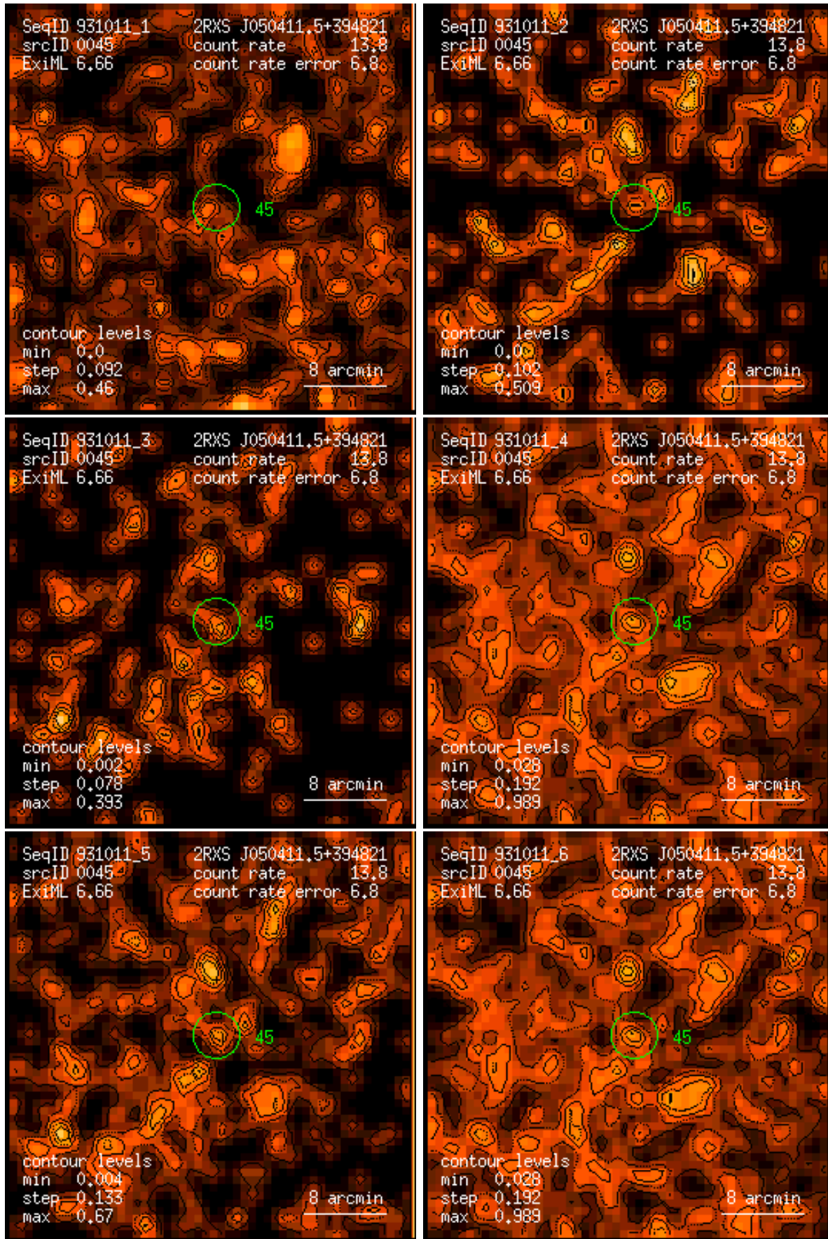
Figure 45: RASS 931011: detection 0045: band rate images, Gaussian filter: (1) PSPC channels 11 – 41, (2) 52 – 90, (3) 91 – 201, (4) 11 – 235, (5) 52 – 201, (6) 11 – 201. Broad band rates in counts/ks. Band rate contour levels in counts/ks/arcmin 2 .
