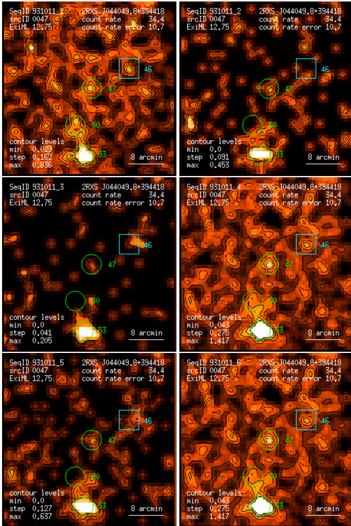
Figure 47: RASS 931011: detection 0047: band rate images, Gaussian filter: (1) PSPC channels 11 – 41, (2) 52 – 90, (3) 91 – 201, (4) 11 – 235, (5) 52 – 201, (6) 11 – 201. Broad band rates in counts/ks. Band rate contour levels in counts/ks/arcmin 2 .
