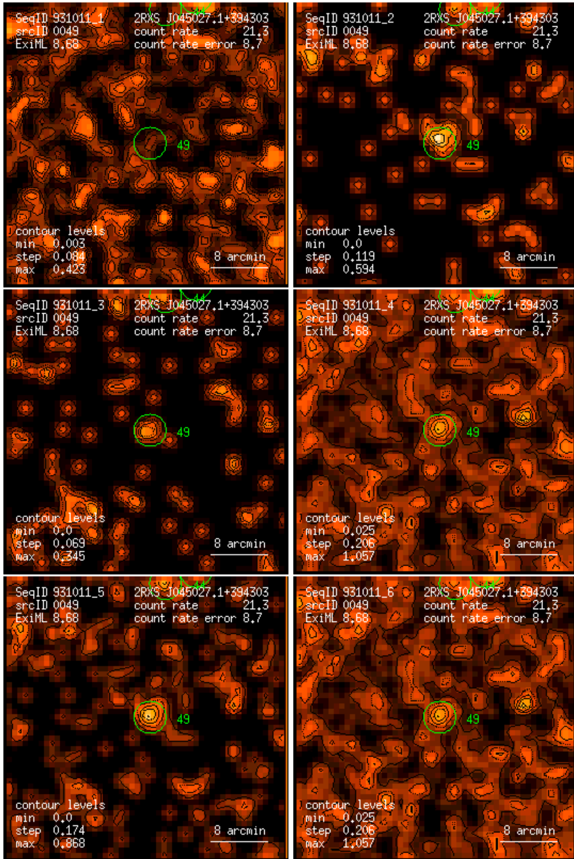
Figure 49: RASS 931011: detection 0049: band rate images, Gaussian filter: (1) PSPC channels 11 – 41, (2) 52 – 90, (3) 91 – 201, (4) 11 – 235, (5) 52 – 201, (6) 11 – 201. Broad band rates in counts/ks. Band rate contour levels in counts/ks/arcmin 2 .
